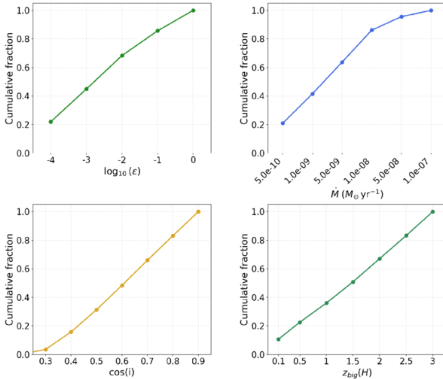
Figure 11. from Ezequiel Manzo-Martínez et al 2026 Astrophys. J. 1006 doi:10.3847/1538-4357/ae8255 https://dx.doi.org/10.3847/1538-4357/ae8255 © 2026. The Author(s). Published by the American Astronomical Society.
