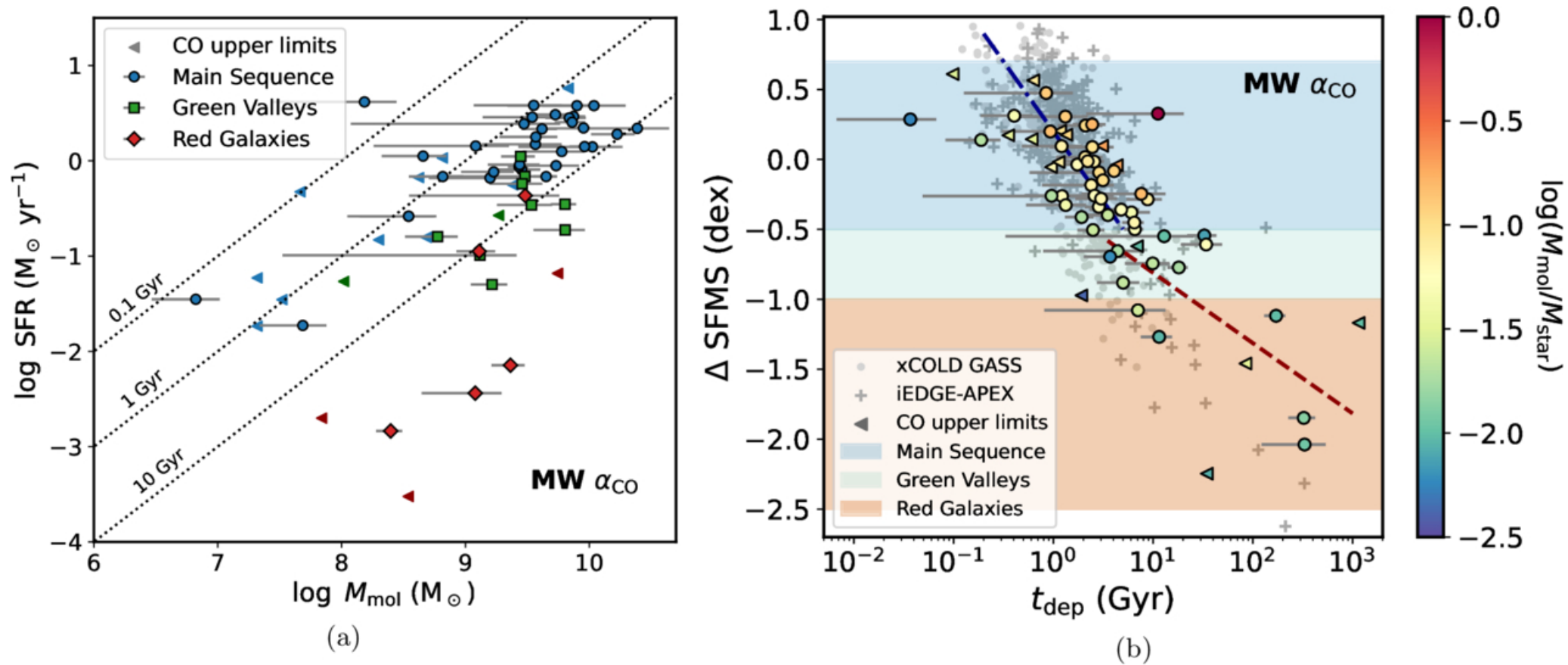
Figure 8. from Yu-Hsuan Teng et al 2026 Astrophys. J. 1007 doi:10.3847/1538-4357/ae81b6 https://dx.doi.org/10.3847/1538-4357/ae81b6 © 2026. The Author(s). Published by the American Astronomical Society.
