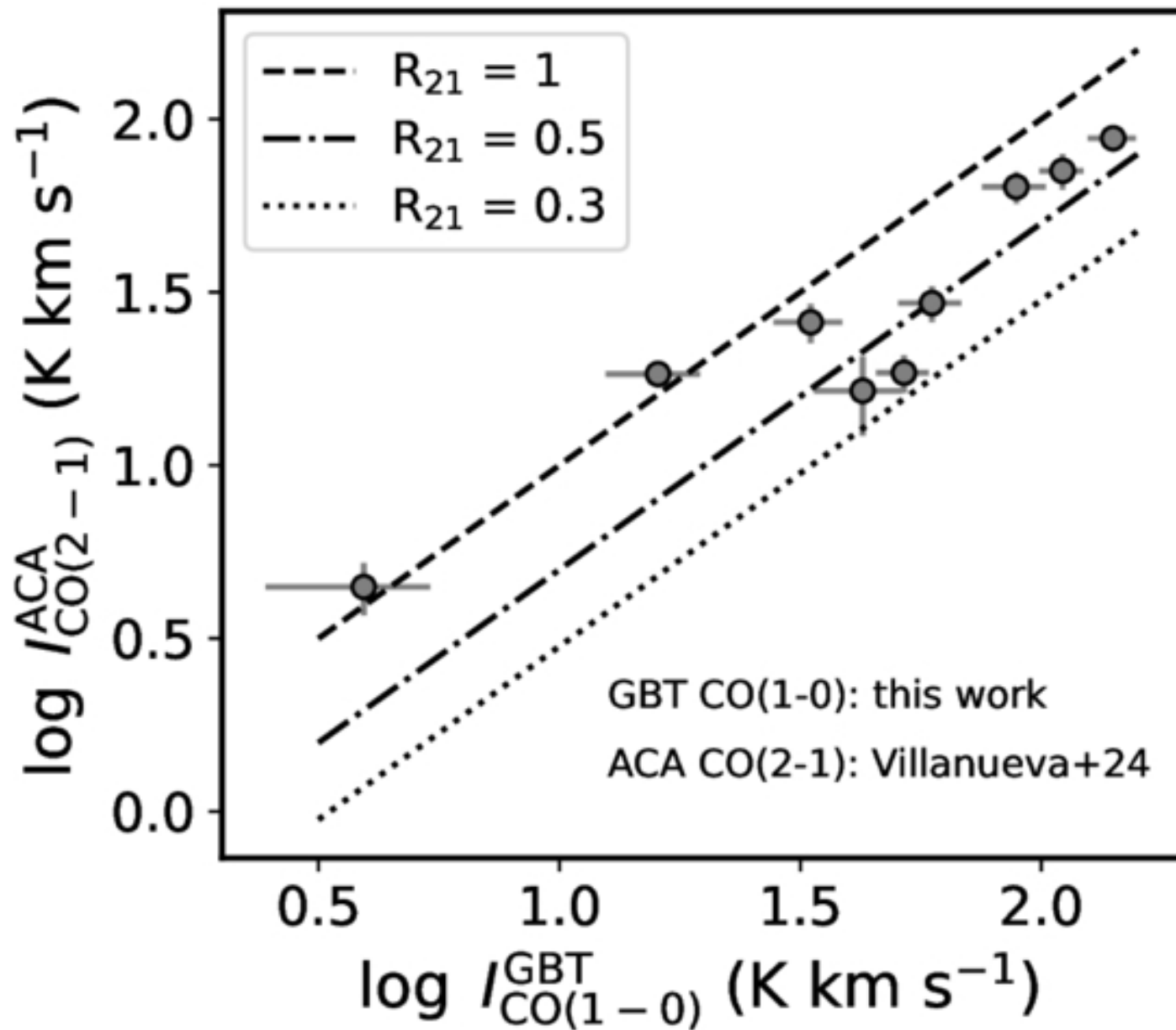
Figure 5. from Yu-Hsuan Teng et al 2026 Astrophys. J. 1007 doi:10.3847/1538-4357/ae81b6 https://dx.doi.org/10.3847/1538-4357/ae81b6 © 2026. The Author(s). Published by the American Astronomical Society.
