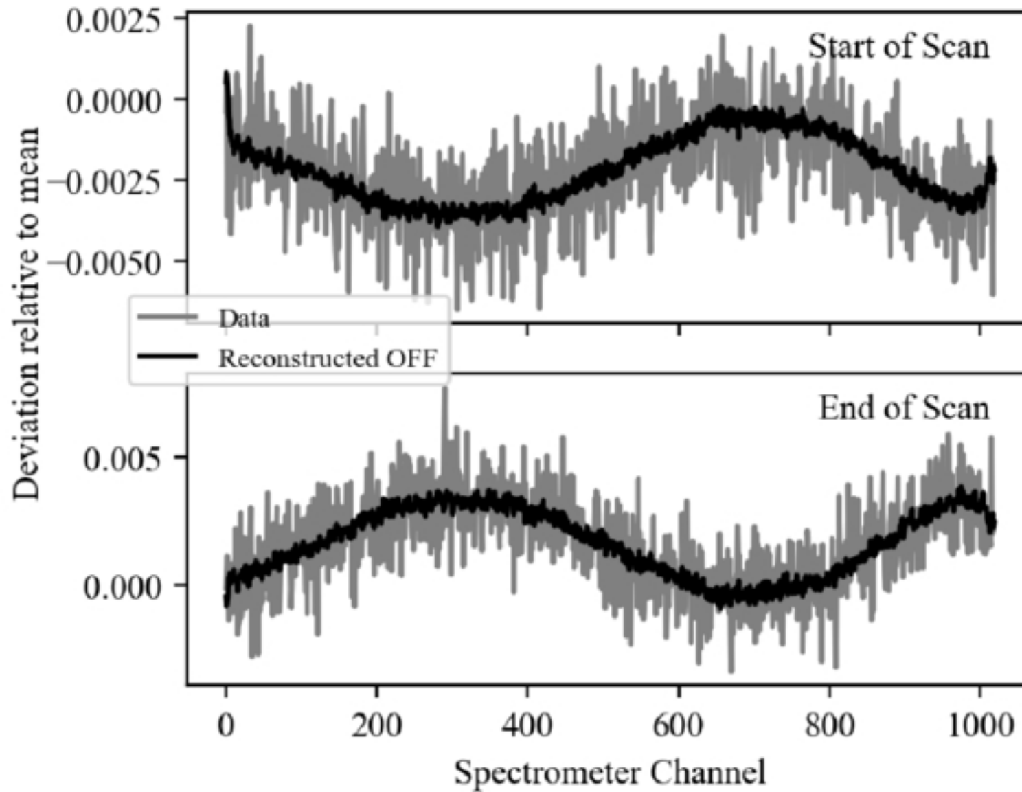
Figure 3. from Yu-Hsuan Teng et al 2026 Astrophys. J. 1007 doi:10.3847/1538-4357/ae81b6 https://dx.doi.org/10.3847/1538-4357/ae81b6 © 2026. The Author(s). Published by the American Astronomical Society.
