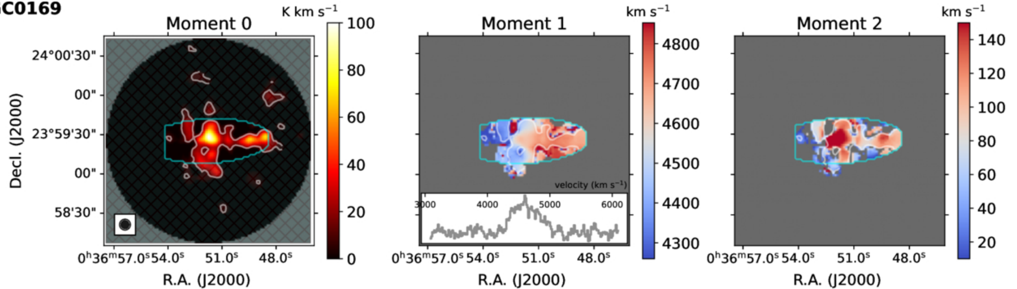
Figure 11. Moment maps and integrated spectra from Yu-Hsuan Teng et al 2026 Astrophys. J. 1007 doi:10.3847/1538-4357/ae81b6 https://dx.doi.org/10.3847/1538-4357/ae81b6 © 2026. The Author(s). Published by the American Astronomical Society.
