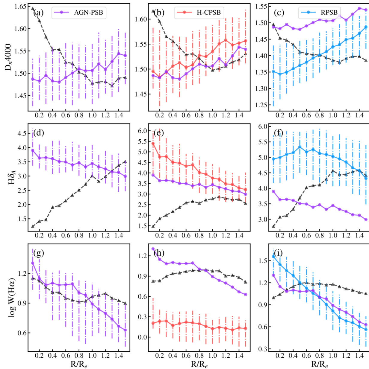
Figure 9. from Junjie Huang et al 2026 Astrophys. J. 1006 doi:10.3847/1538-4357/ae81b0 https://dx.doi.org/10.3847/1538-4357/ae81b0 © 2026. The Author(s). Published by the American Astronomical Society.
