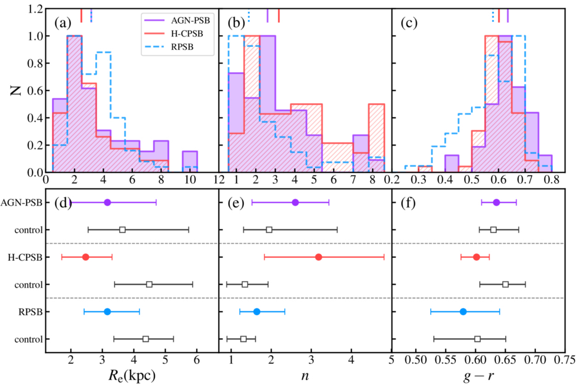
Figure 8. from Junjie Huang et al 2026 Astrophys. J. 1006 doi:10.3847/1538-4357/ae81b0 https://dx.doi.org/10.3847/1538-4357/ae81b0 © 2026. The Author(s). Published by the American Astronomical Society.
