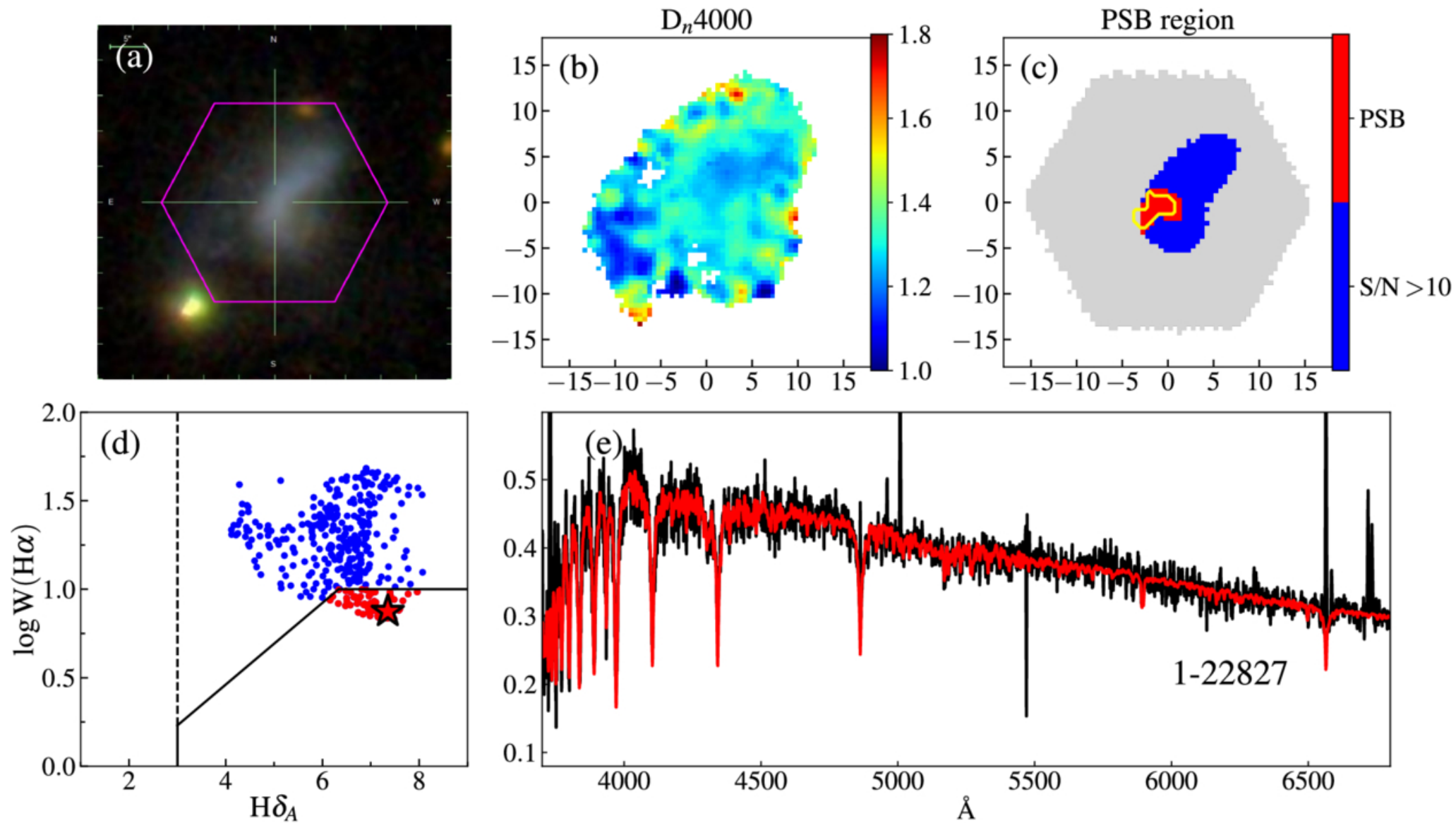
Figure 7. from Junjie Huang et al 2026 Astrophys. J. 1006 doi:10.3847/1538-4357/ae81b0 https://dx.doi.org/10.3847/1538-4357/ae81b0 © 2026. The Author(s). Published by the American Astronomical Society.
