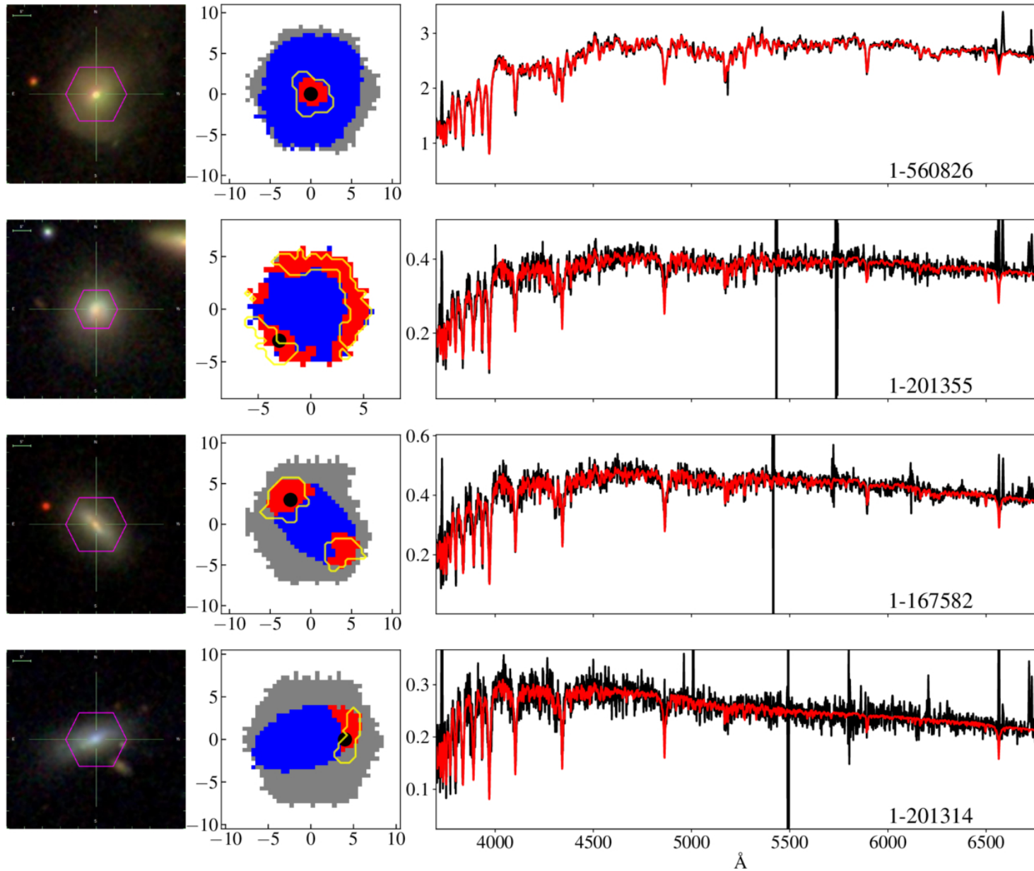
Figure 2. from Junjie Huang et al 2026 Astrophys. J. 1006 doi:10.3847/1538-4357/ae81b0 https://dx.doi.org/10.3847/1538-4357/ae81b0 © 2026. The Author(s). Published by the American Astronomical Society.
