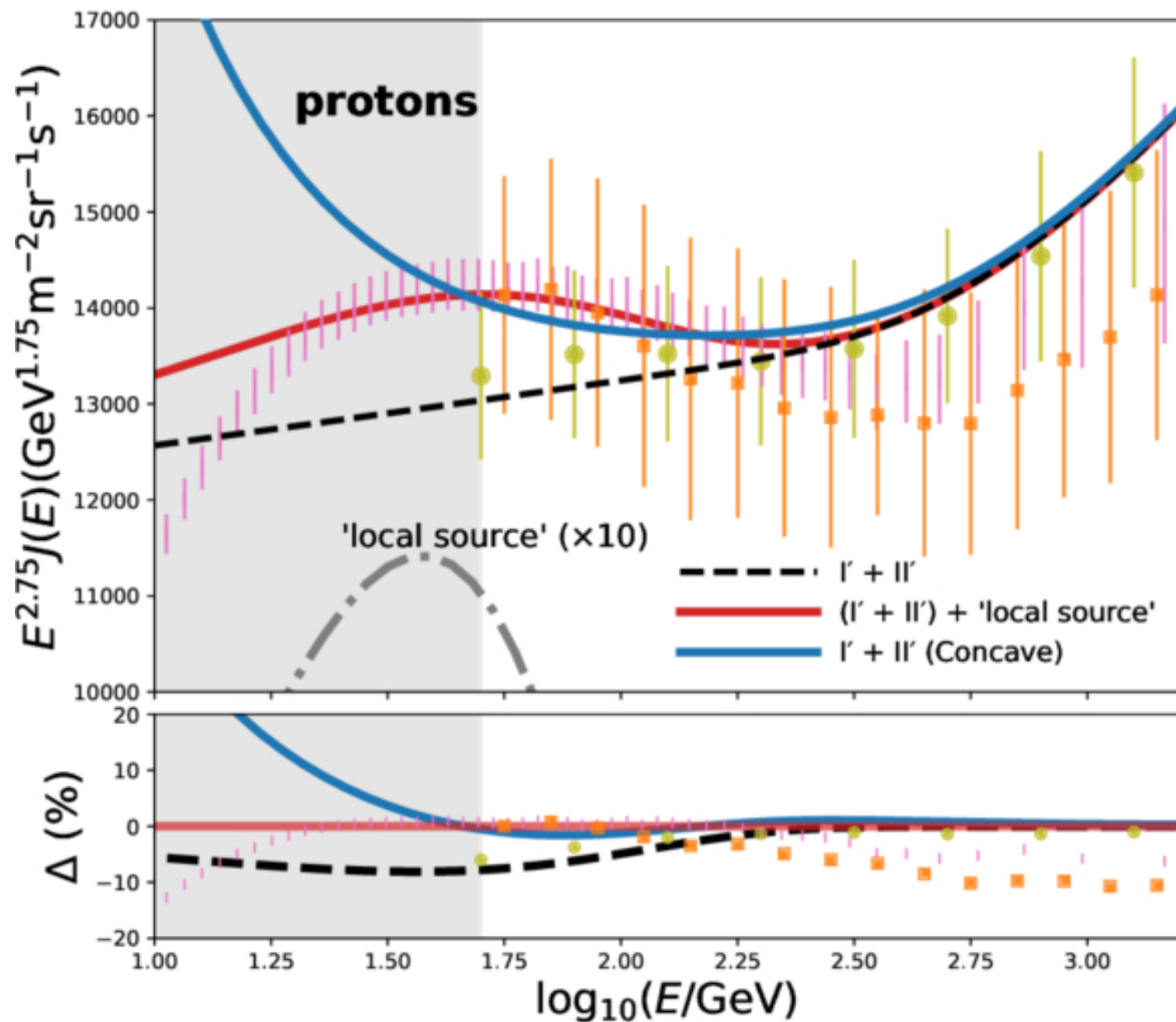
Figure 7. from Felix Aharonian and Bing Theodore Zhang 2026 Astrophys. J. 1006 doi:10.3847/1538-4357/ae81a7 https://dx.doi.org/10.3847/1538-4357/ae81a7 © 2026. The Author(s). Published by the American Astronomical Society.
