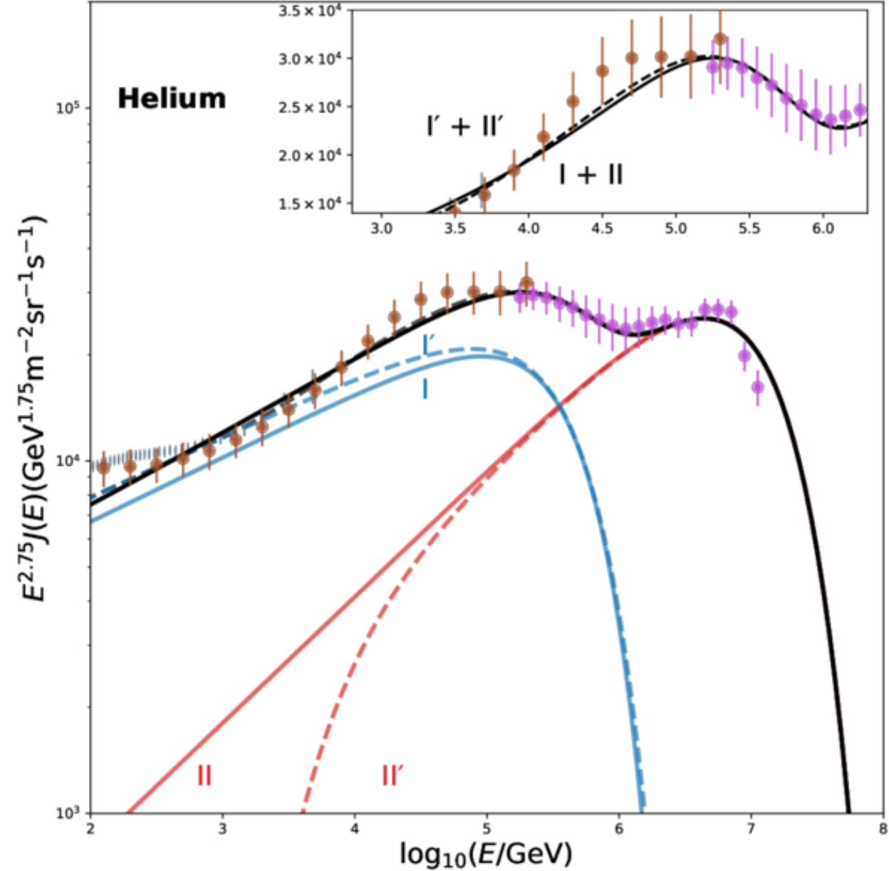
Figure 5. from Felix Aharonian and Bing Theodore Zhang 2026 Astrophys. J. 1006 doi:10.3847/1538-4357/ae81a7 https://dx.doi.org/10.3847/1538-4357/ae81a7 © 2026. The Author(s). Published by the American Astronomical Society.
