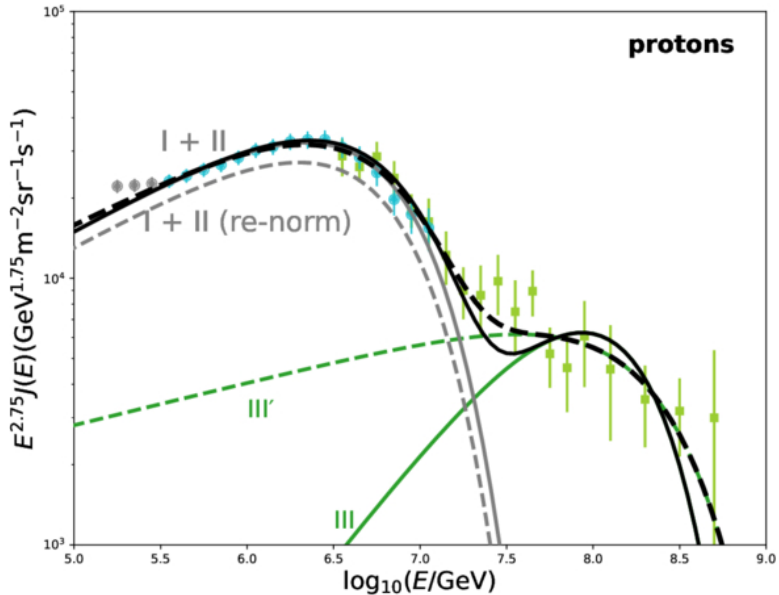
Figure 3. from Felix Aharonian and Bing Theodore Zhang 2026 Astrophys. J. 1006 doi:10.3847/1538-4357/ae81a7 https://dx.doi.org/10.3847/1538-4357/ae81a7 © 2026. The Author(s). Published by the American Astronomical Society.
