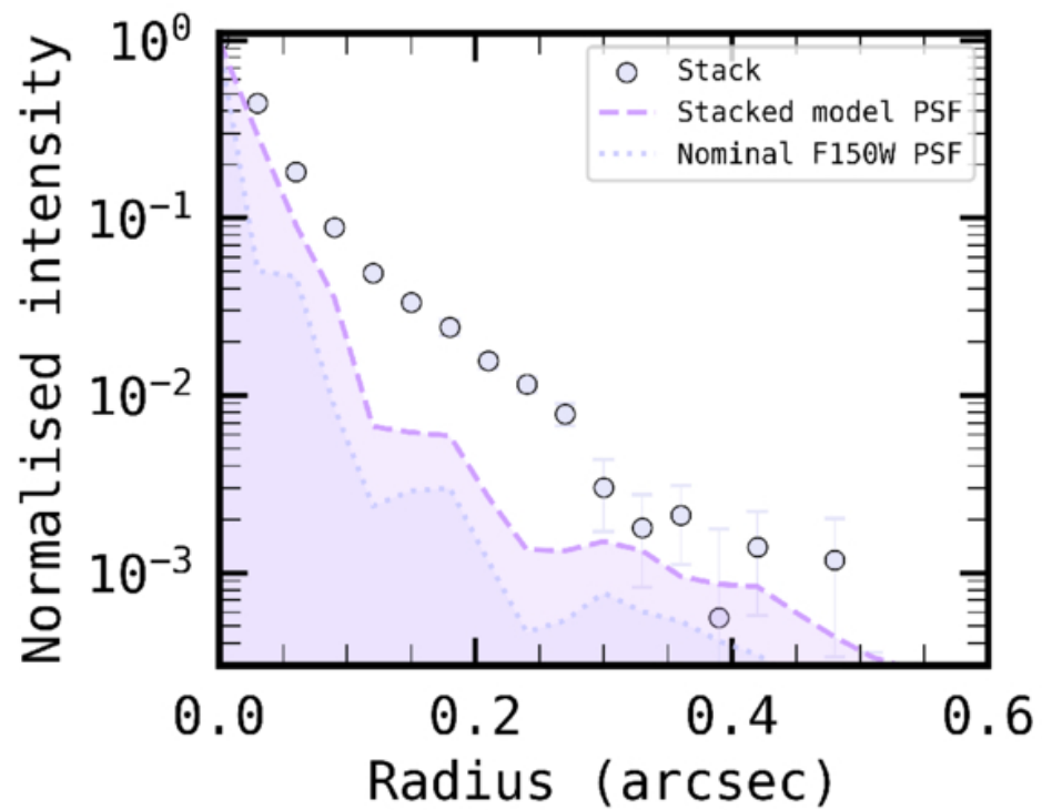
Figure 7. from Pierluigi Rinaldi et al 2026 Astrophys. J. 1006 doi:10.3847/1538-4357/ae80cd https://dx.doi.org/10.3847/1538-4357/ae80cd © 2026. The Author(s). Published by the American Astronomical Society.
