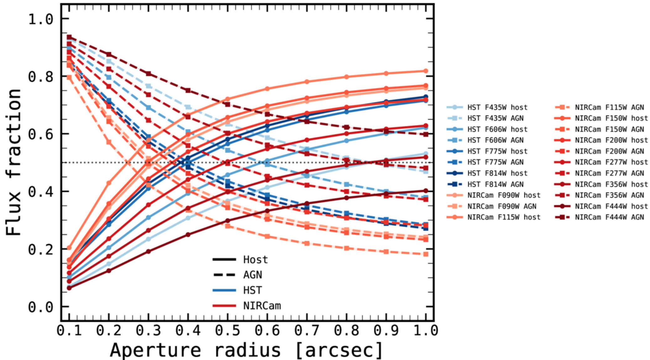
Figure 12. from Pierluigi Rinaldi et al 2026 Astrophys. J. 1006 doi:10.3847/1538-4357/ae80cd https://dx.doi.org/10.3847/1538-4357/ae80cd © 2026. The Author(s). Published by the American Astronomical Society.
