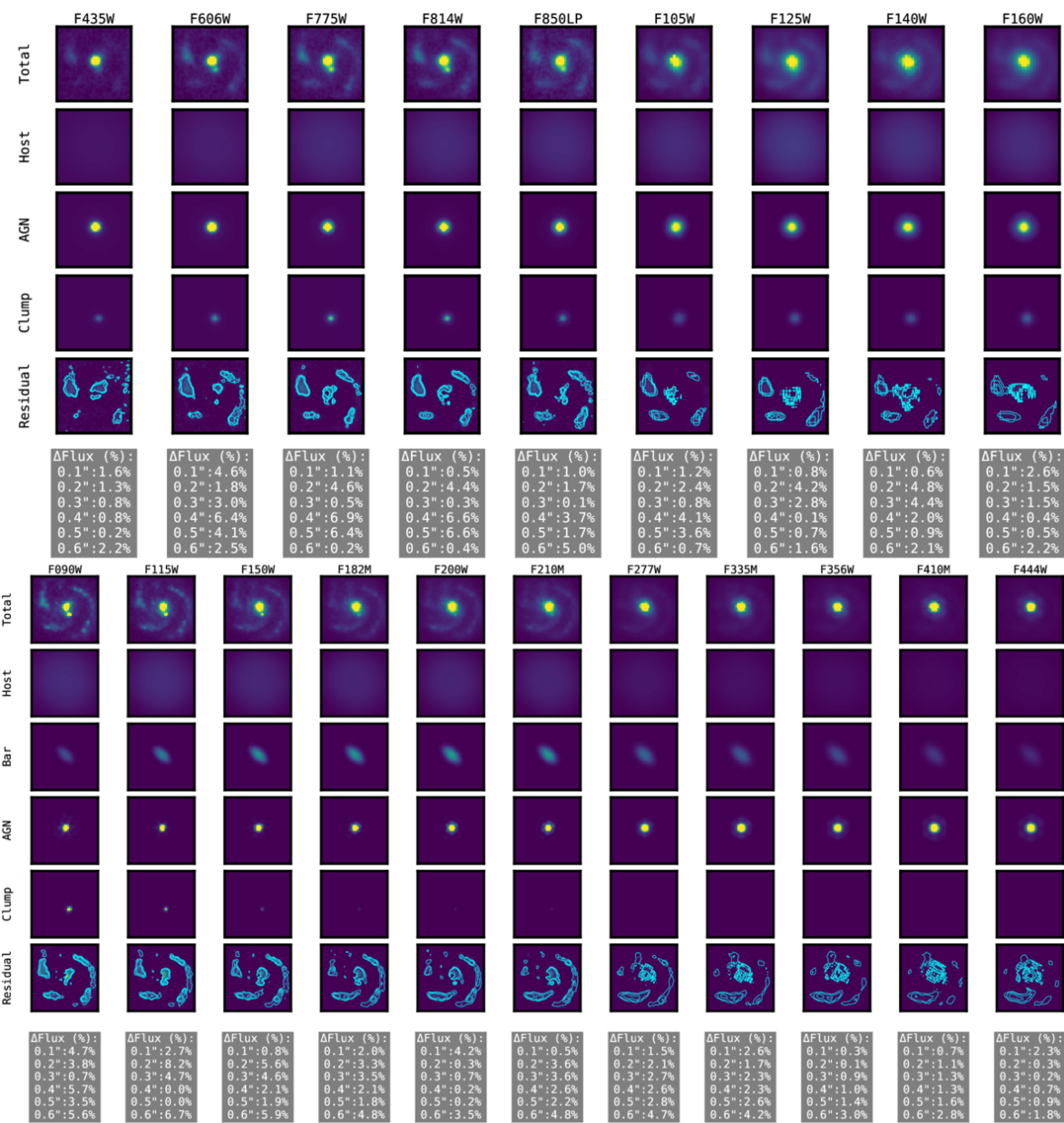
Figure 11. from Pierluigi Rinaldi et al 2026 Astrophys. J. 1006 doi:10.3847/1538-4357/ae80cd https://dx.doi.org/10.3847/1538-4357/ae80cd © 2026. The Author(s). Published by the American Astronomical Society.
