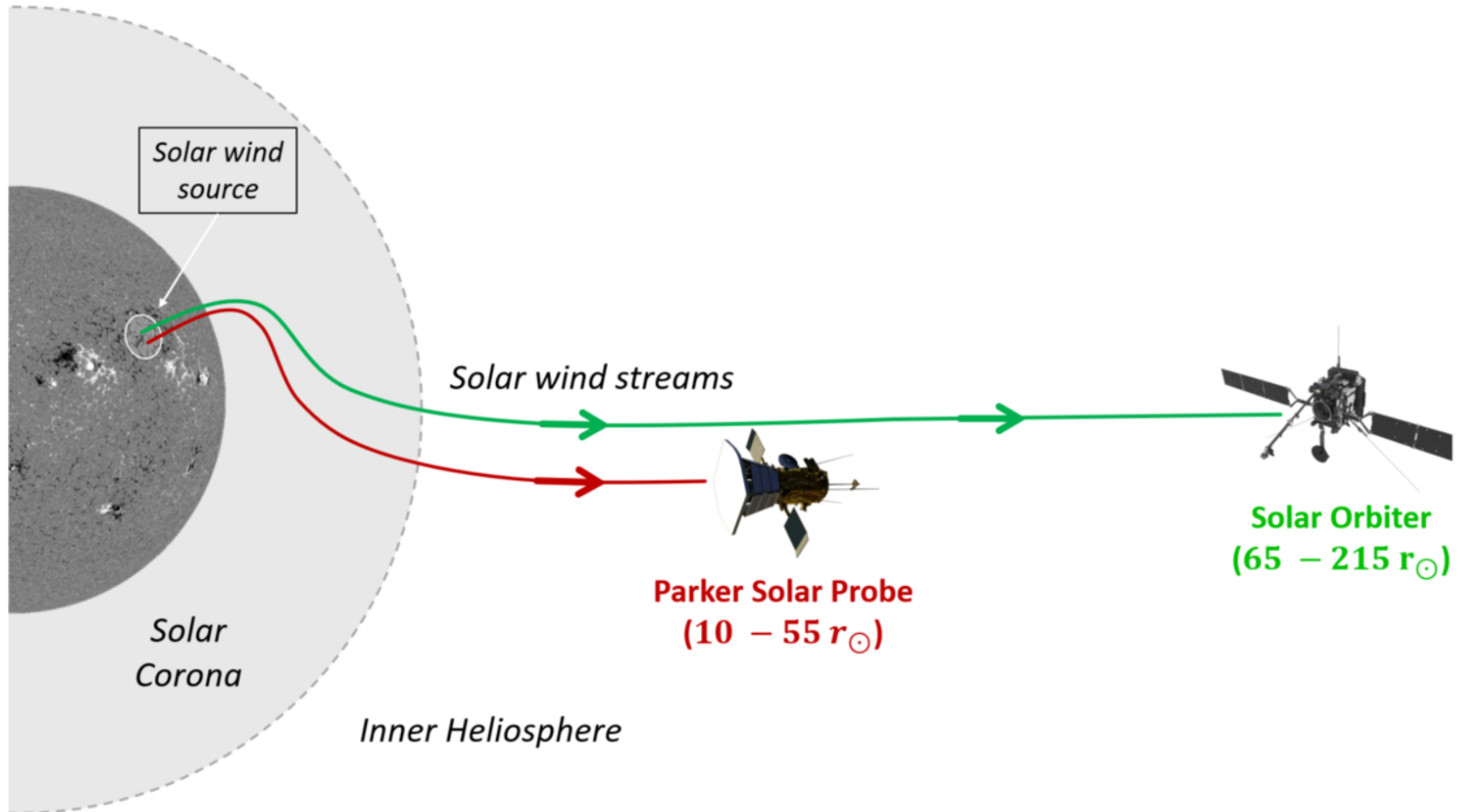
Figure 1. from Jean-Baptiste Dakeyo et al 2026 Astrophys. J. 1006 doi:10.3847/1538-4357/ae80a4 https://dx.doi.org/10.3847/1538-4357/ae80a4 © 2026. The Author(s). Published by the American Astronomical Society.
