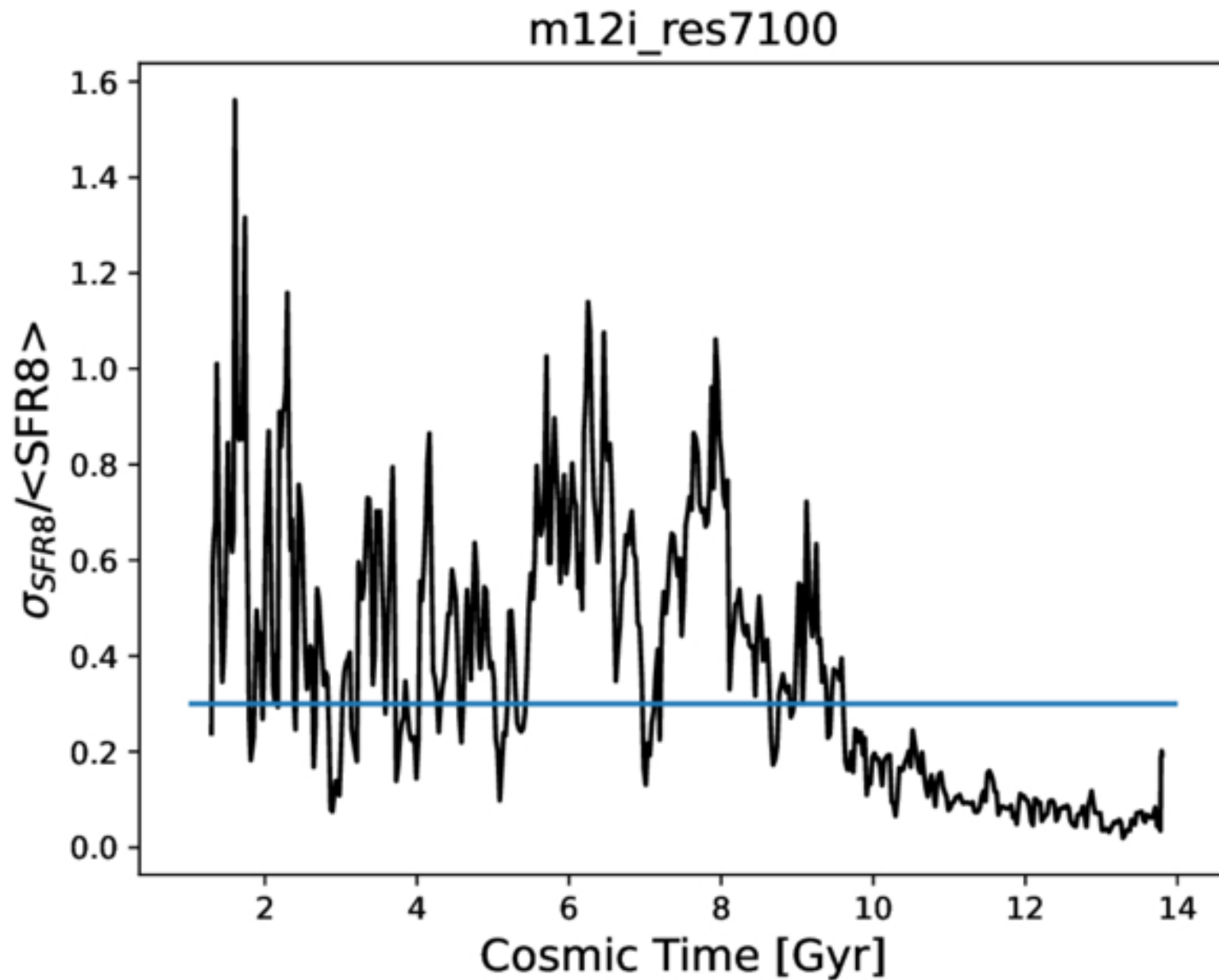
Figure 7. from Fraser M. Smith and Robert J. Thacker 2026 Astrophys. J. 1006 doi:10.3847/1538-4357/ae80a1 https://dx.doi.org/10.3847/1538-4357/ae80a1 © 2026. The Author(s). Published by the American Astronomical Society.
