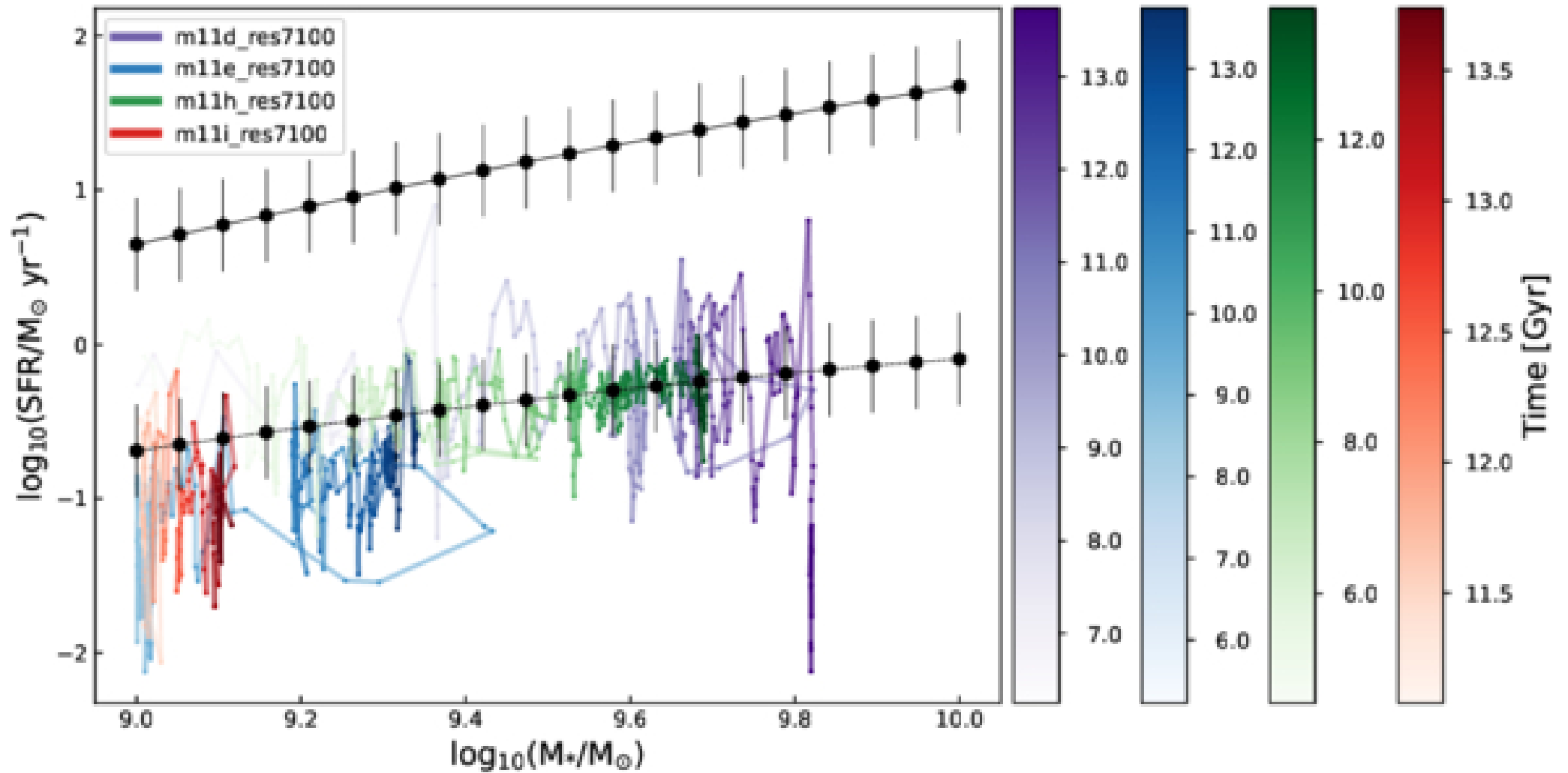
Figure 3. from Fraser M. Smith and Robert J. Thacker 2026 Astrophys. J. 1006 doi:10.3847/1538-4357/ae80a1 https://dx.doi.org/10.3847/1538-4357/ae80a1 © 2026. The Author(s). Published by the American Astronomical Society.
