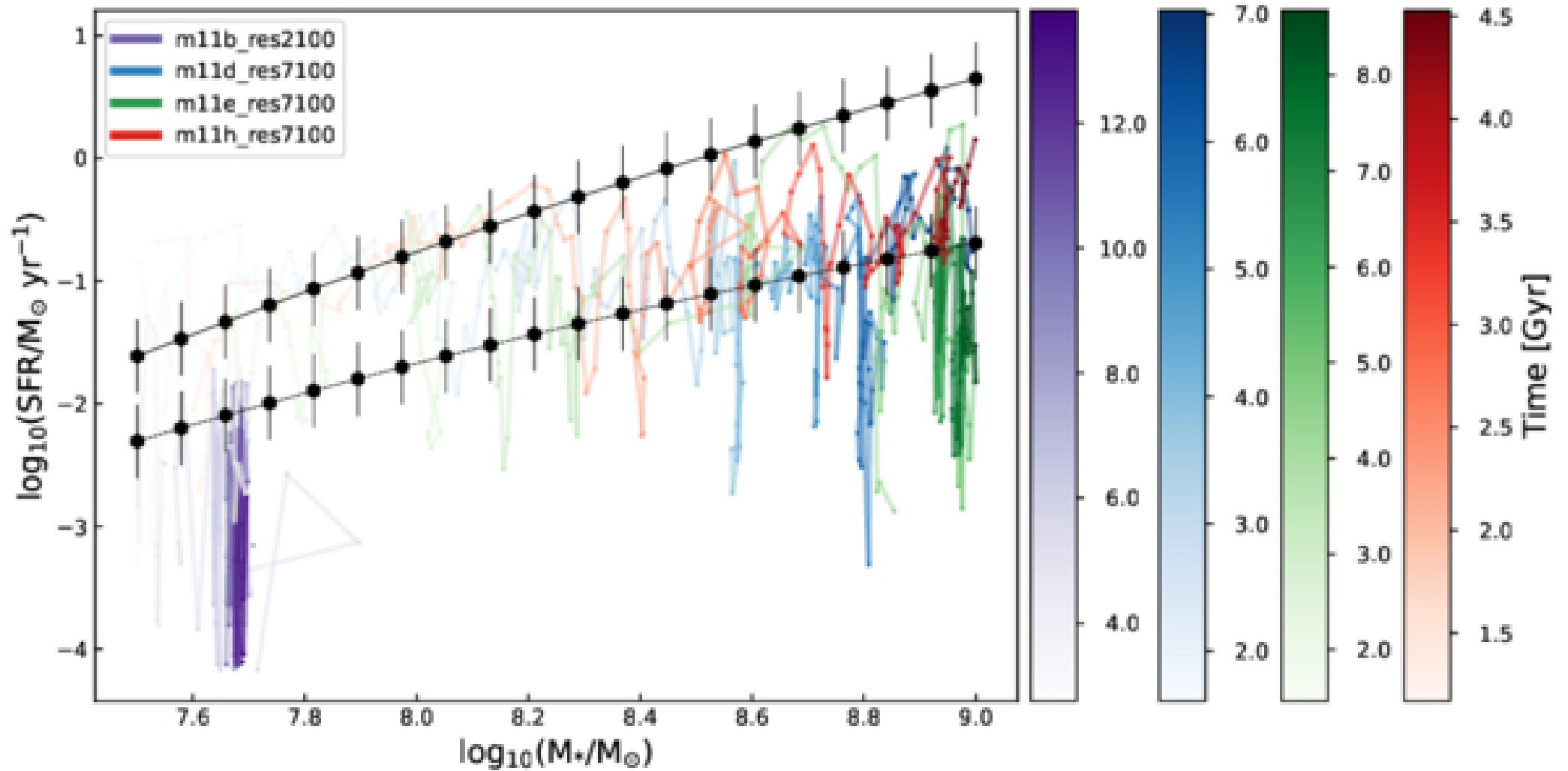
Figure 2. from Fraser M. Smith and Robert J. Thacker 2026 Astrophys. J. 1006 doi:10.3847/1538-4357/ae80a1 https://dx.doi.org/10.3847/1538-4357/ae80a1 © 2026. The Author(s). Published by the American Astronomical Society.
