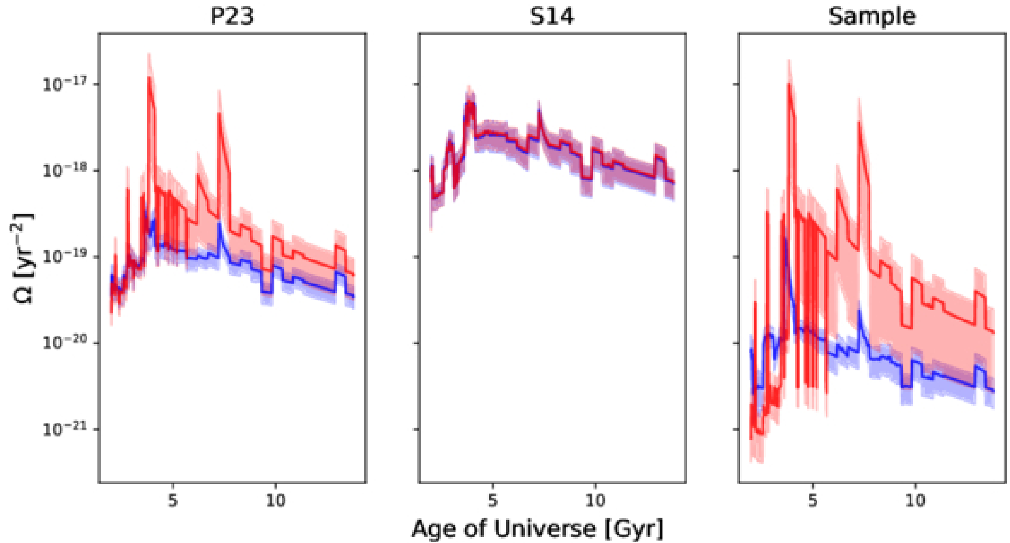
Figure 11. from Fraser M. Smith and Robert J. Thacker 2026 Astrophys. J. 1006 doi:10.3847/1538-4357/ae80a1 https://dx.doi.org/10.3847/1538-4357/ae80a1 © 2026. The Author(s). Published by the American Astronomical Society.
