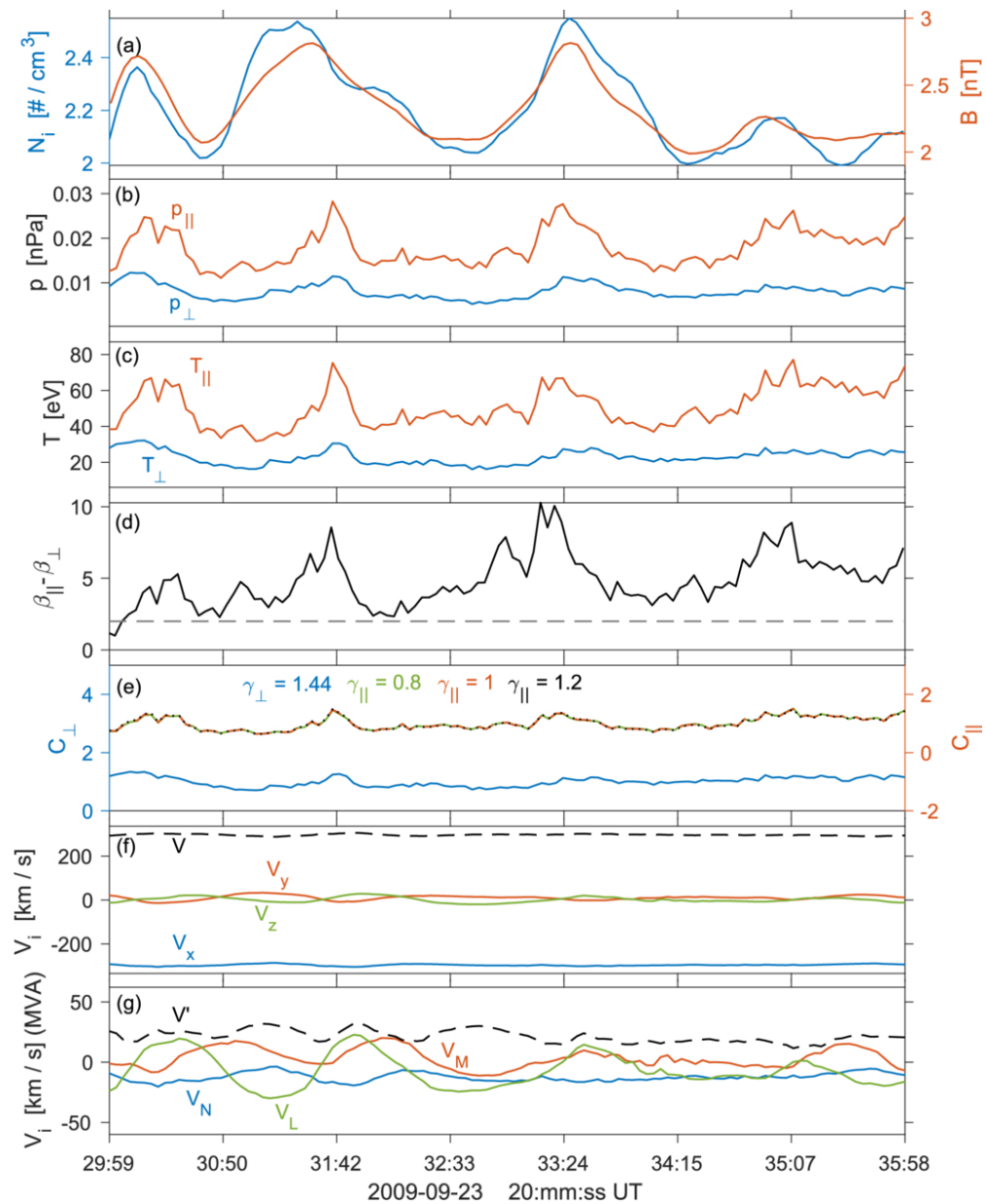
Figure 4. from L.-N. Hau et al 2026 Astrophys. J. 1006 doi:10.3847/1538-4357/ae809b https://dx.doi.org/10.3847/1538-4357/ae809b © 2026. The Author(s). Published by the American Astronomical Society.
