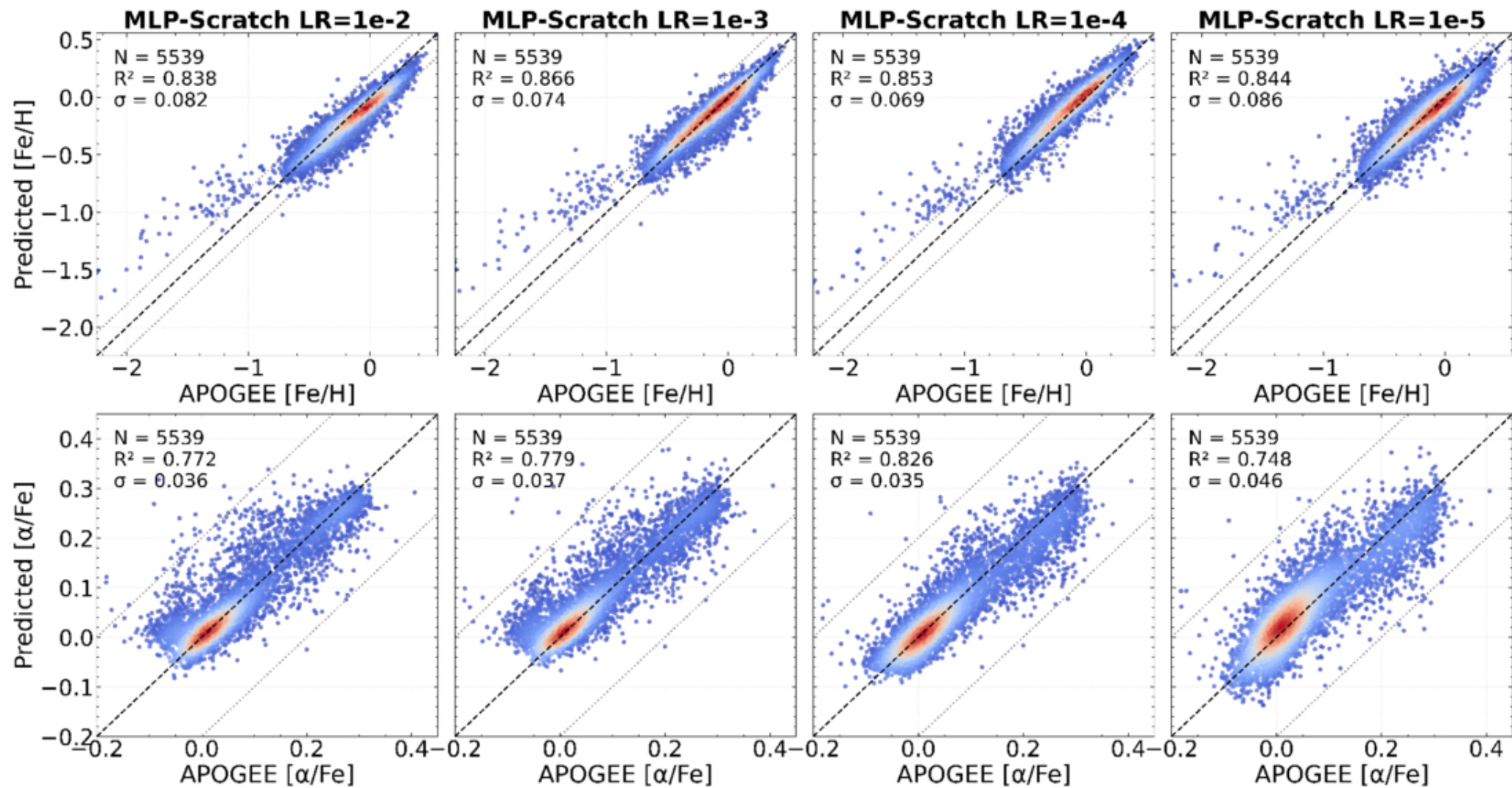
Figure A4. from Xiaosheng Zhao et al 2026 Astrophys. J. 1006 doi:10.3847/1538-4357/ae7f0a https://dx.doi.org/10.3847/1538-4357/ae7f0a © 2026. The Author(s). Published by the American Astronomical Society.
