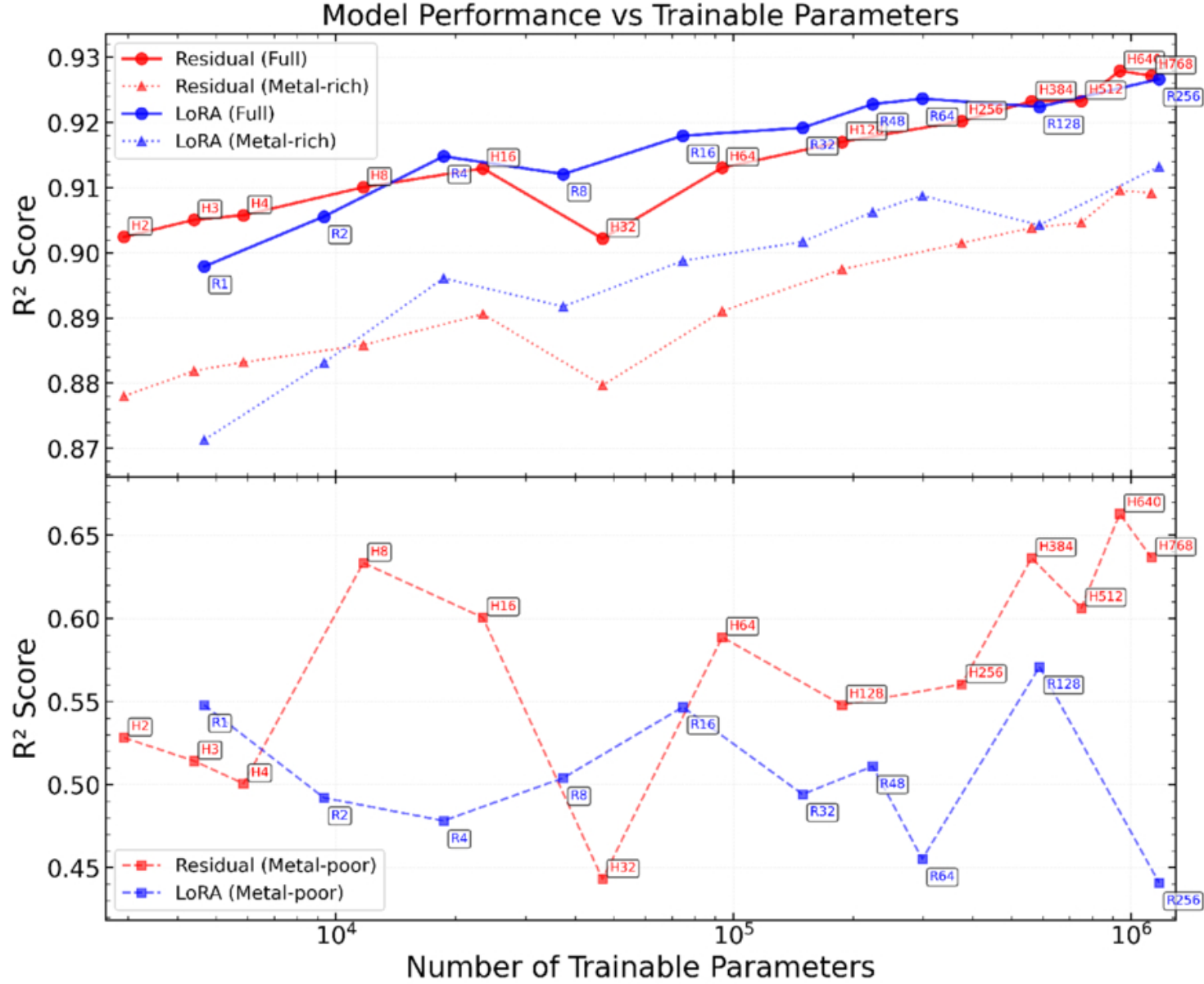
Figure A3. from Xiaosheng Zhao et al 2026 Astrophys. J. 1006 doi:10.3847/1538-4357/ae7f0a https://dx.doi.org/10.3847/1538-4357/ae7f0a © 2026. The Author(s). Published by the American Astronomical Society.
