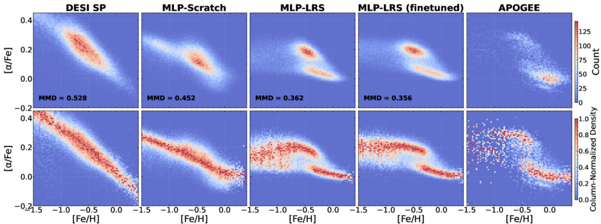
Figure 3. from Xiaosheng Zhao et al 2026 Astrophys. J. 1006 doi:10.3847/1538-4357/ae7f0a https://dx.doi.org/10.3847/1538-4357/ae7f0a © 2026. The Author(s). Published by the American Astronomical Society.
