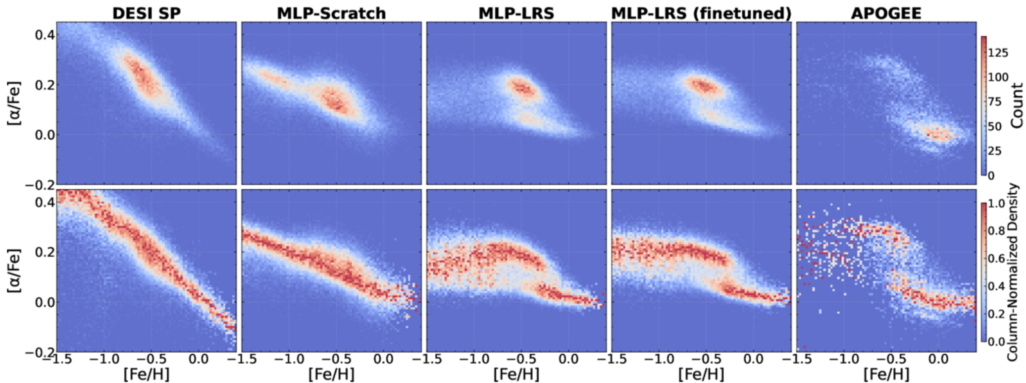
Figure D2. from Xiaosheng Zhao et al 2026 Astrophys. J. 1006 doi:10.3847/1538-4357/ae7f0a https://dx.doi.org/10.3847/1538-4357/ae7f0a © 2026. The Author(s). Published by the American Astronomical Society.
