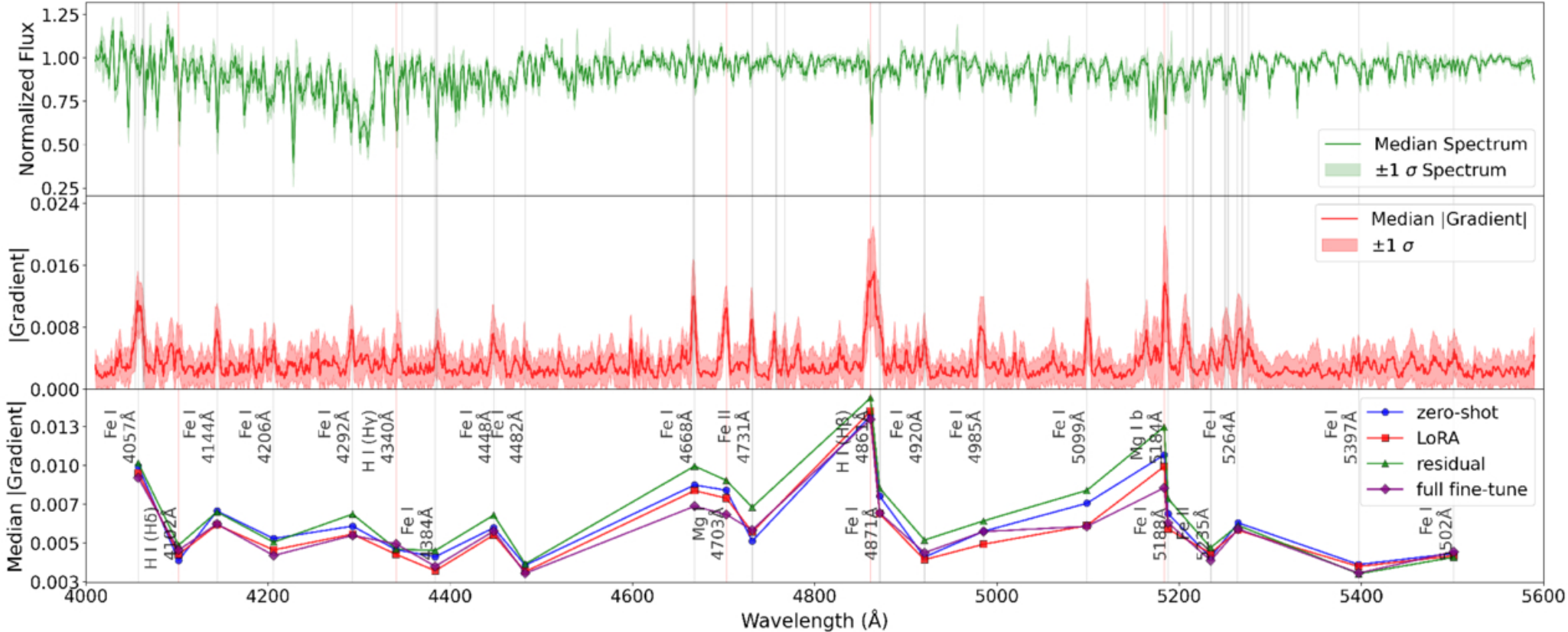
Figure B1. from Xiaosheng Zhao et al 2026 Astrophys. J. 1006 doi:10.3847/1538-4357/ae7f0a https://dx.doi.org/10.3847/1538-4357/ae7f0a © 2026. The Author(s). Published by the American Astronomical Society.
