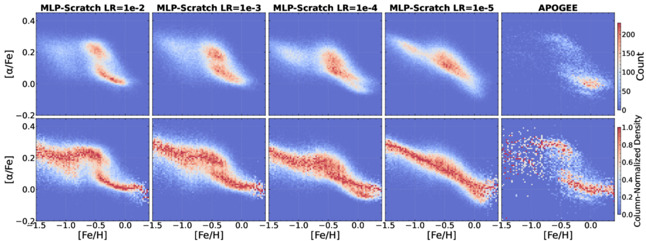
Figure A5. from Xiaosheng Zhao et al 2026 Astrophys. J. 1006 doi:10.3847/1538-4357/ae7f0a https://dx.doi.org/10.3847/1538-4357/ae7f0a © 2026. The Author(s). Published by the American Astronomical Society.
