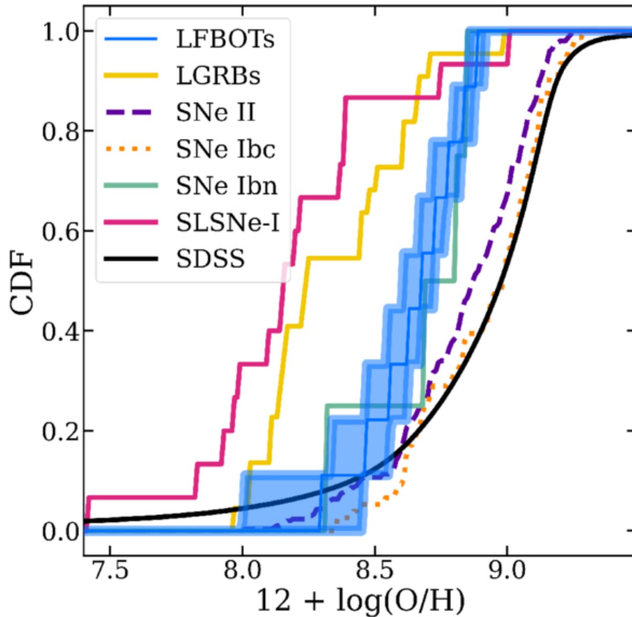
Figure 4. from Anya E. Nugent et al 2026 Astrophys. J. 1006 doi:10.3847/1538-4357/ae7e77 https://dx.doi.org/10.3847/1538-4357/ae7e77 © 2026. The Author(s). Published by the American Astronomical Society.
