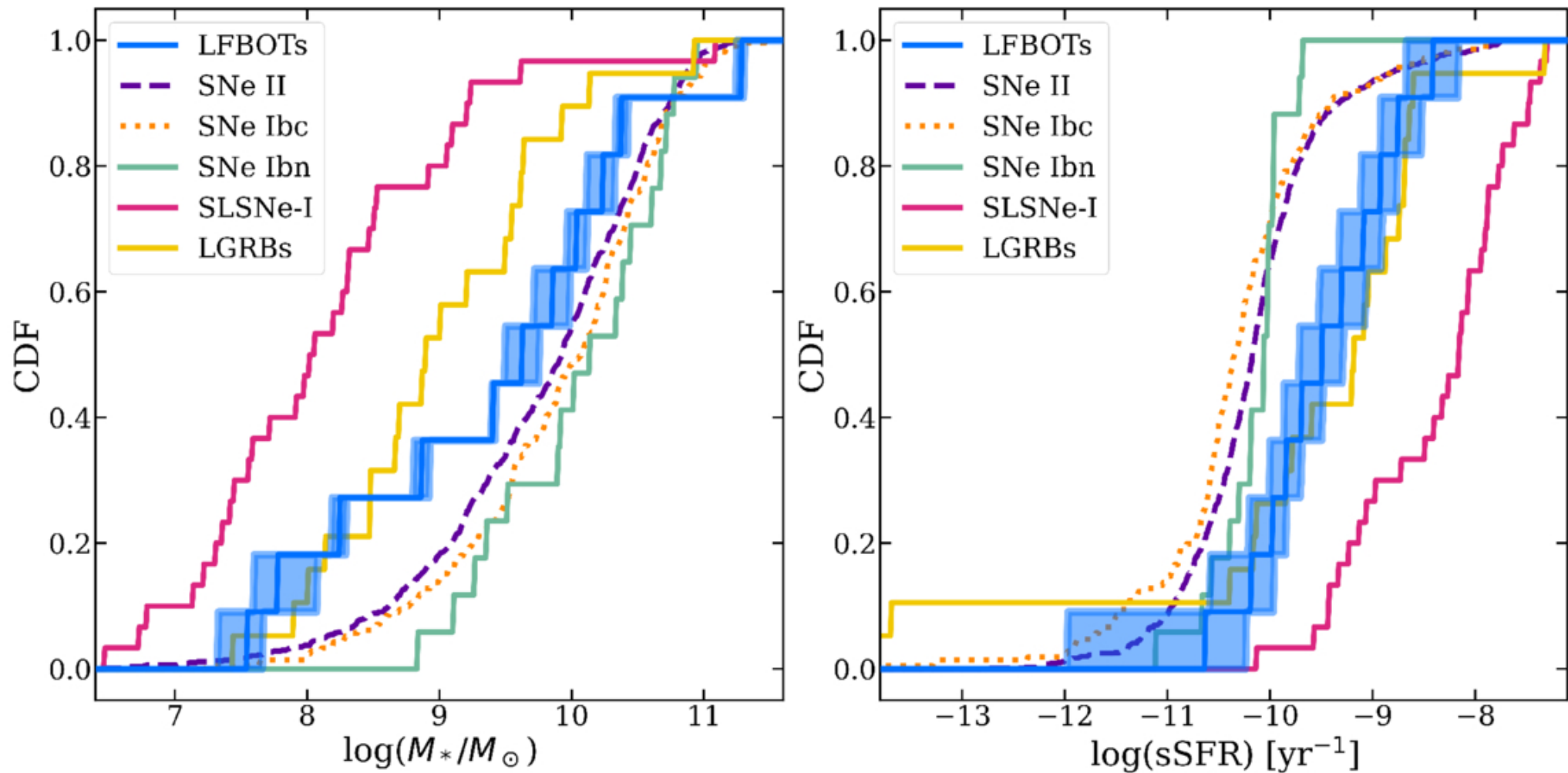
Figure 2. from Anya E. Nugent et al 2026 Astrophys. J. 1006 doi:10.3847/1538-4357/ae7e77 https://dx.doi.org/10.3847/1538-4357/ae7e77 © 2026. The Author(s). Published by the American Astronomical Society.
