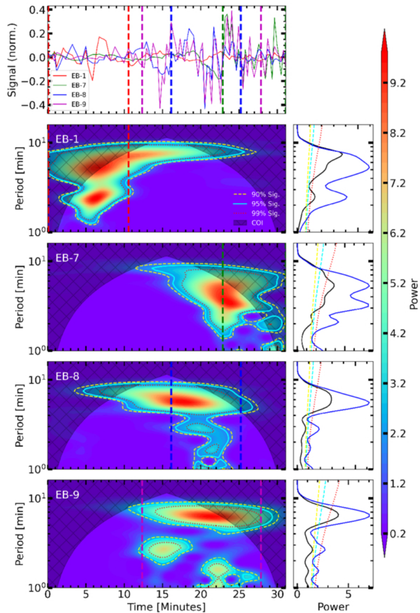
Figure 9. from Ravi Chaurasiya et al 2026 Astrophys. J. 1006 doi:10.3847/1538-4357/ae7dea https://dx.doi.org/10.3847/1538-4357/ae7dea © 2026. The Author(s). Published by the American Astronomical Society.
