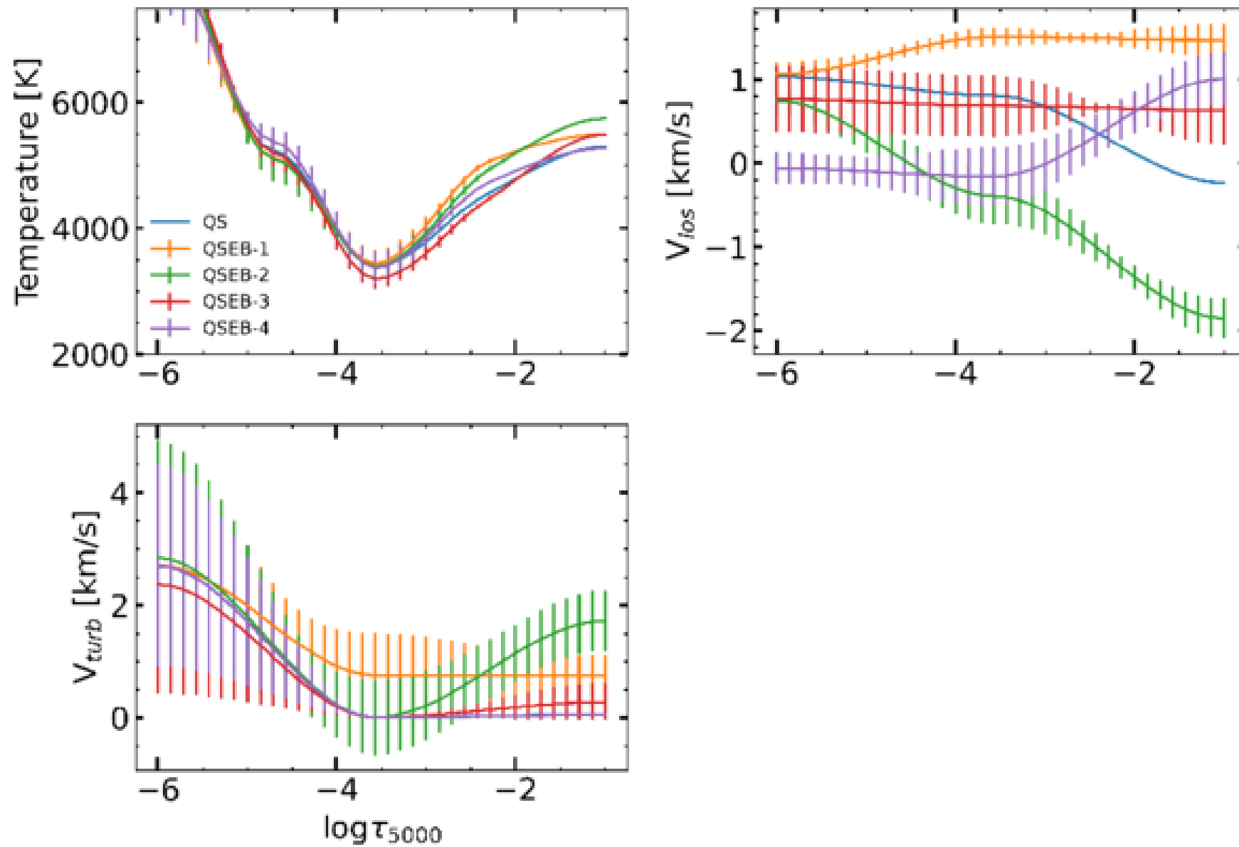
Figure 8. from Ravi Chaurasiya et al 2026 Astrophys. J. 1006 doi:10.3847/1538-4357/ae7dea https://dx.doi.org/10.3847/1538-4357/ae7dea © 2026. The Author(s). Published by the American Astronomical Society.
