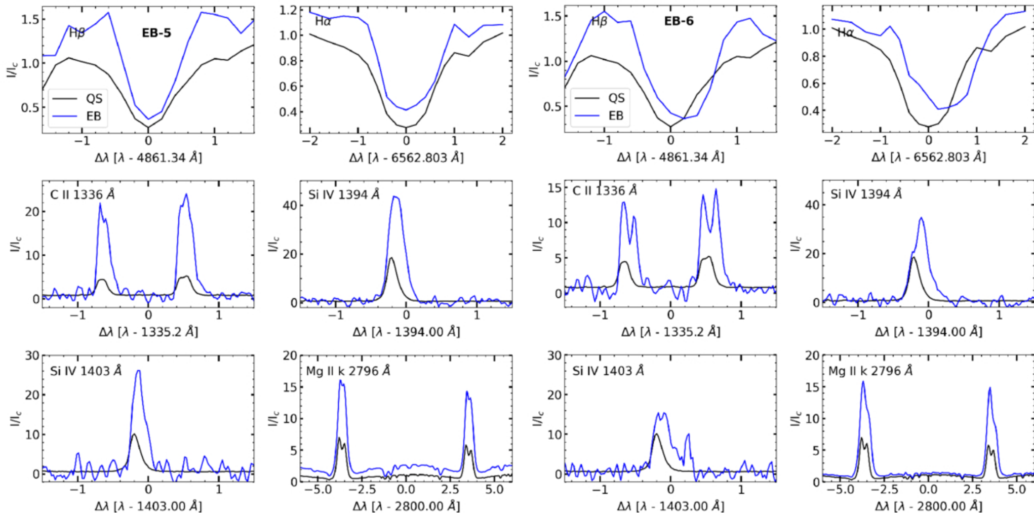
Figure 6. from Ravi Chaurasiya et al 2026 Astrophys. J. 1006 doi:10.3847/1538-4357/ae7dea https://dx.doi.org/10.3847/1538-4357/ae7dea © 2026. The Author(s). Published by the American Astronomical Society.
