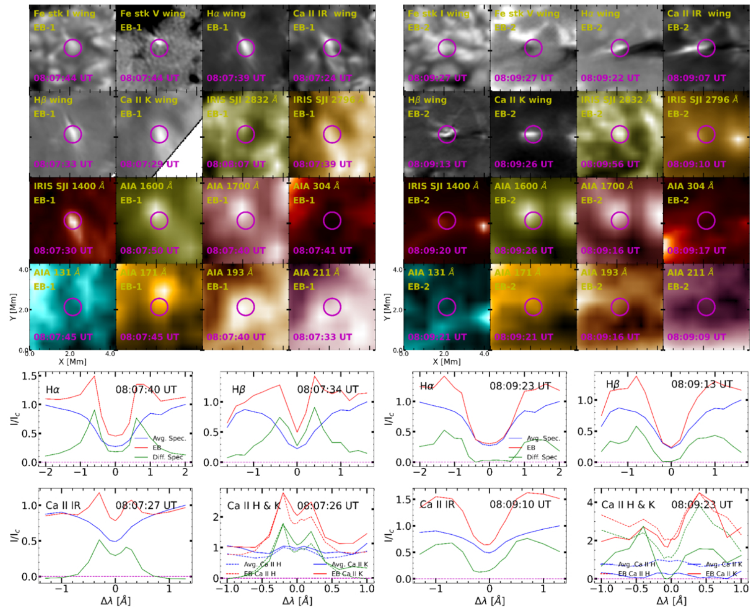
Figure 3. from Ravi Chaurasiya et al 2026 Astrophys. J. 1006 doi:10.3847/1538-4357/ae7dea https://dx.doi.org/10.3847/1538-4357/ae7dea © 2026. The Author(s). Published by the American Astronomical Society.
