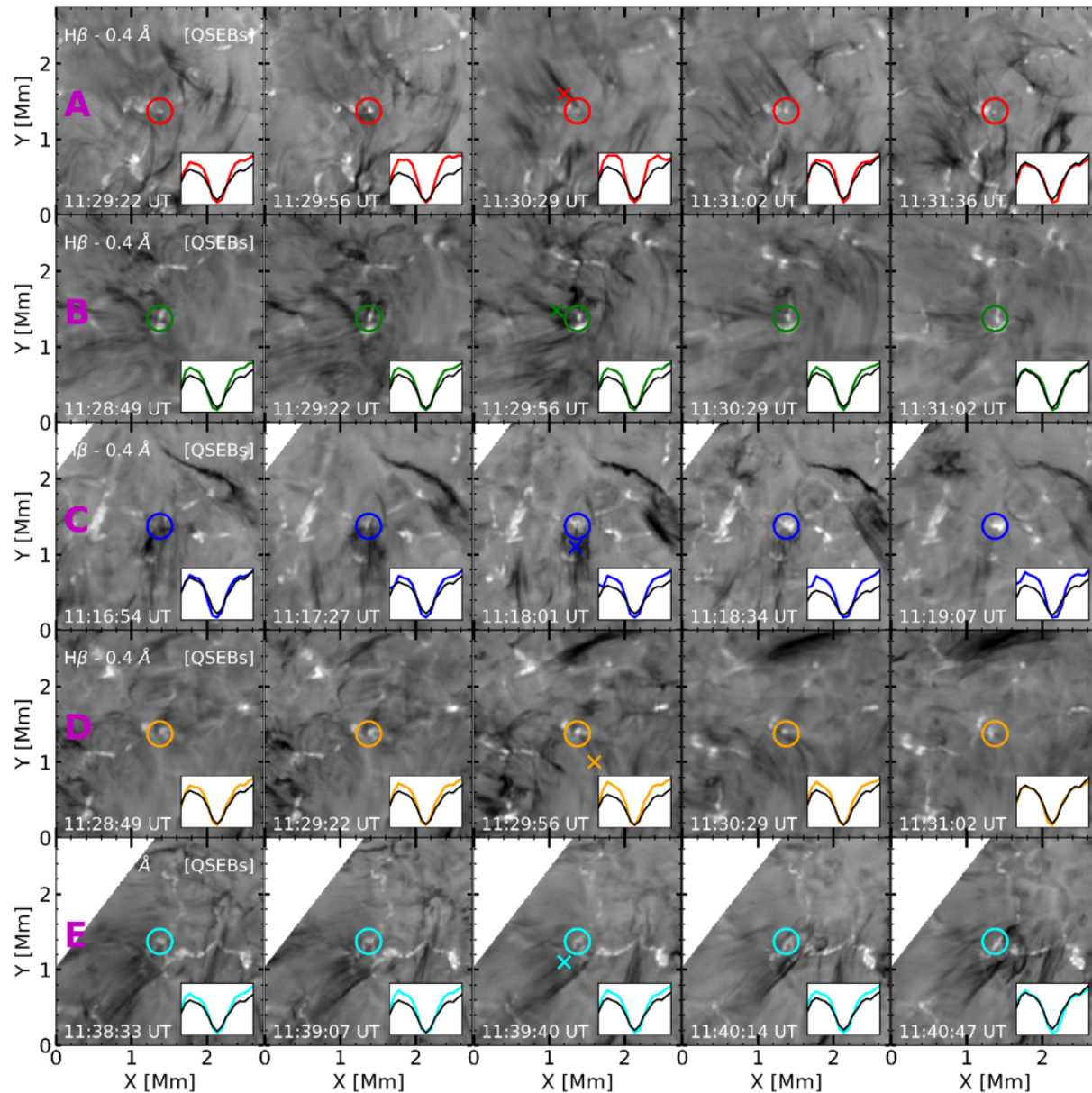
Figure 11. from Ravi Chaurasiya et al 2026 Astrophys. J. 1006 doi:10.3847/1538-4357/ae7dea https://dx.doi.org/10.3847/1538-4357/ae7dea © 2026. The Author(s). Published by the American Astronomical Society.
