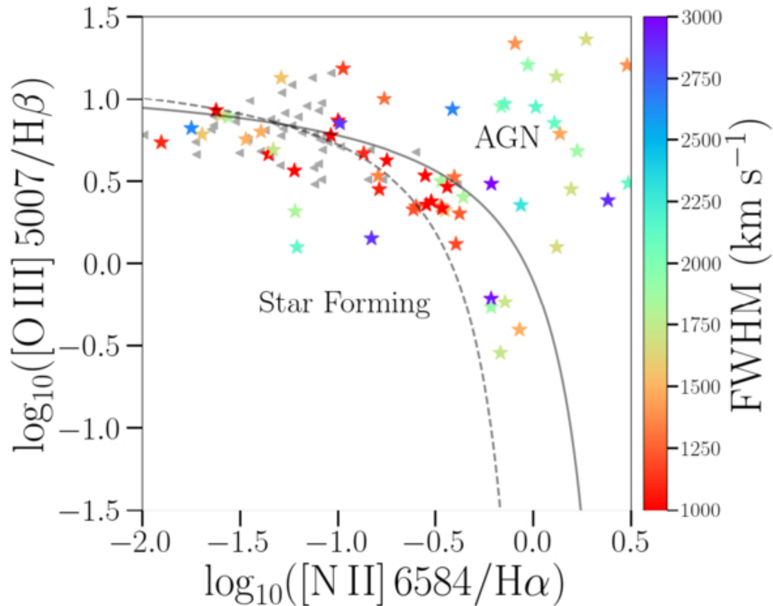
Figure 6. from Caroline J. Baccus and Xinfeng Xu 2026 Astrophys. J. 1006 doi:10.3847/1538-4357/ae7de7 https://dx.doi.org/10.3847/1538-4357/ae7de7 © 2026. The Author(s). Published by the American Astronomical Society.
