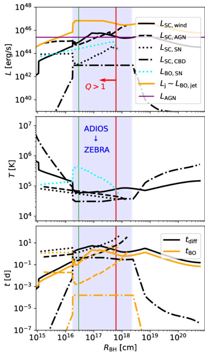
Figure 8. from Hiromichi Tagawa et al 2026 Astrophys. J. 1006 doi:10.3847/1538-4357/ae7d29 https://dx.doi.org/10.3847/1538-4357/ae7d29 © 2026. The Author(s). Published by the American Astronomical Society.
