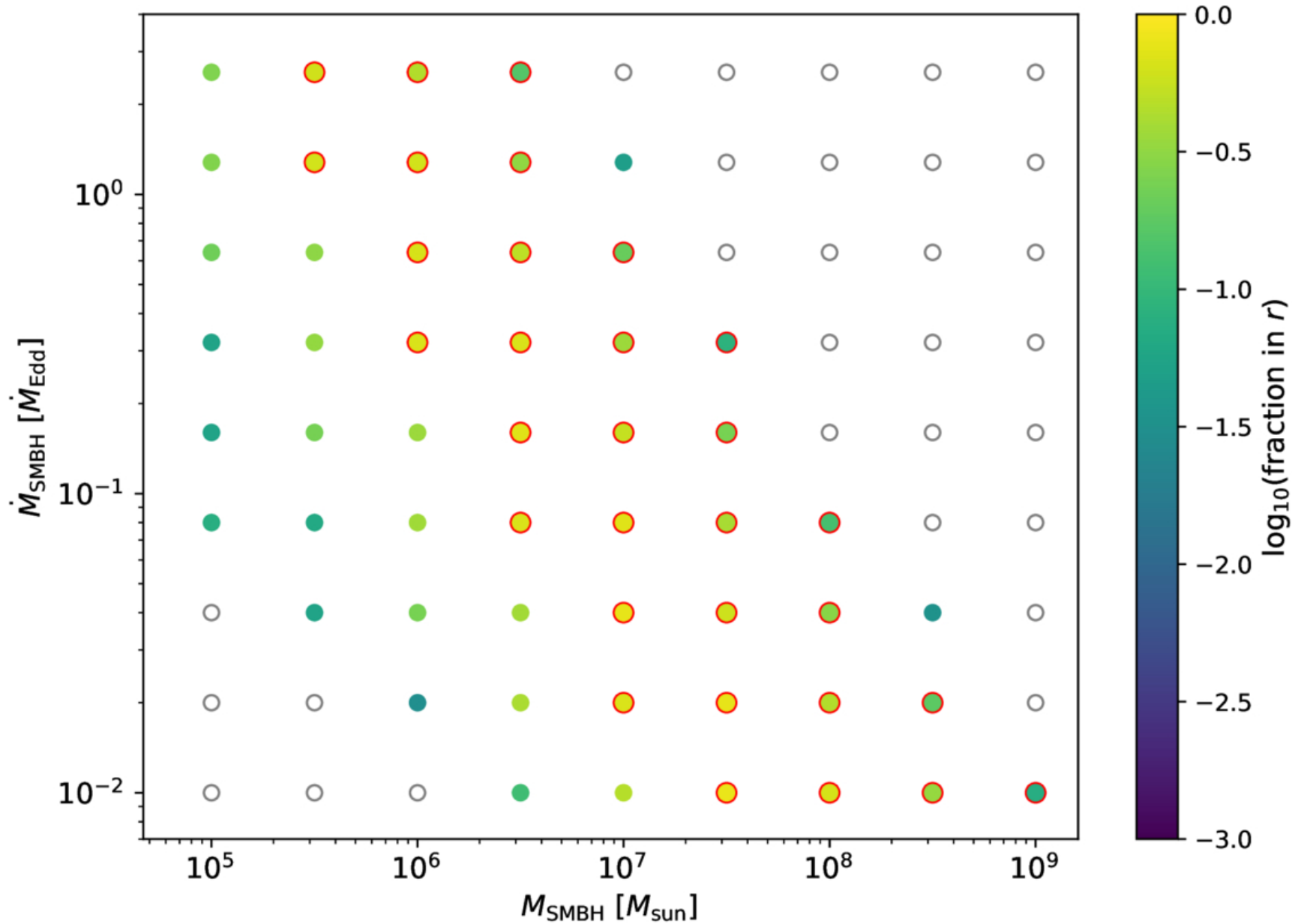
Figure 7. from Hiromichi Tagawa et al 2026 Astrophys. J. 1006 doi:10.3847/1538-4357/ae7d29 https://dx.doi.org/10.3847/1538-4357/ae7d29 © 2026. The Author(s). Published by the American Astronomical Society.
