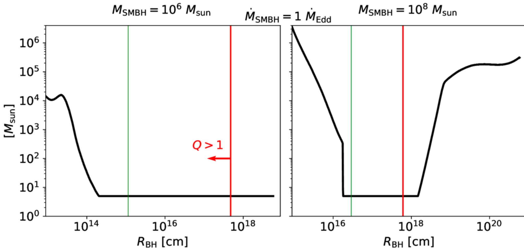
Figure 4. from Hiromichi Tagawa et al 2026 Astrophys. J. 1006 doi:10.3847/1538-4357/ae7d29 https://dx.doi.org/10.3847/1538-4357/ae7d29 © 2026. The Author(s). Published by the American Astronomical Society.
