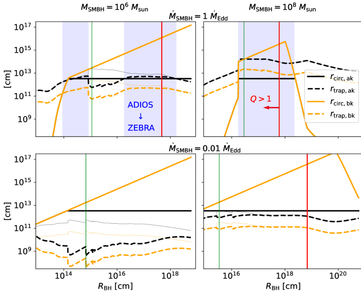
Figure 2. from Hiromichi Tagawa et al 2026 Astrophys. J. 1006 doi:10.3847/1538-4357/ae7d29 https://dx.doi.org/10.3847/1538-4357/ae7d29 © 2026. The Author(s). Published by the American Astronomical Society.
