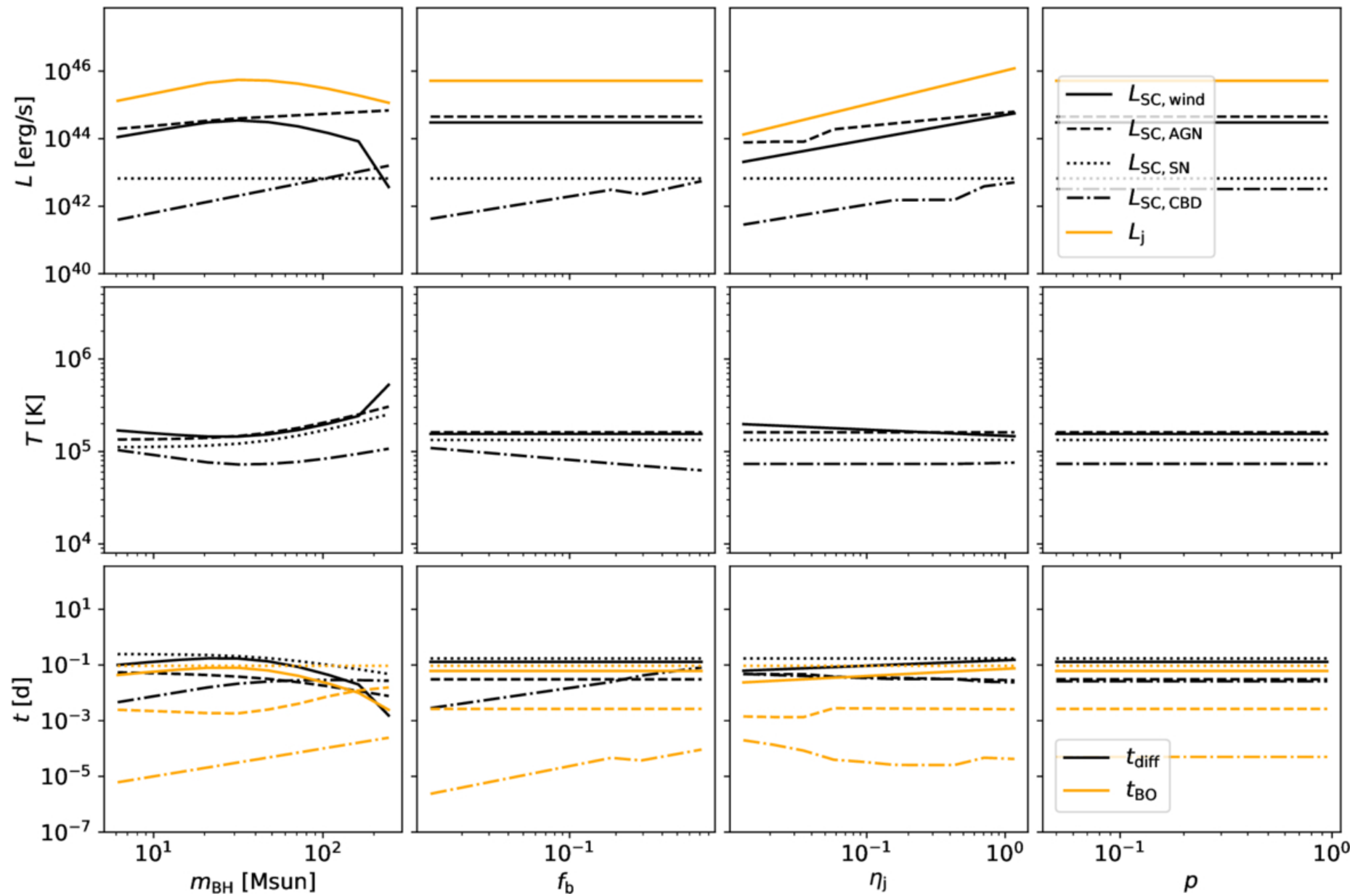
Figure 15. from Hiromichi Tagawa et al 2026 Astrophys. J. 1006 doi:10.3847/1538-4357/ae7d29 https://dx.doi.org/10.3847/1538-4357/ae7d29 © 2026. The Author(s). Published by the American Astronomical Society.
