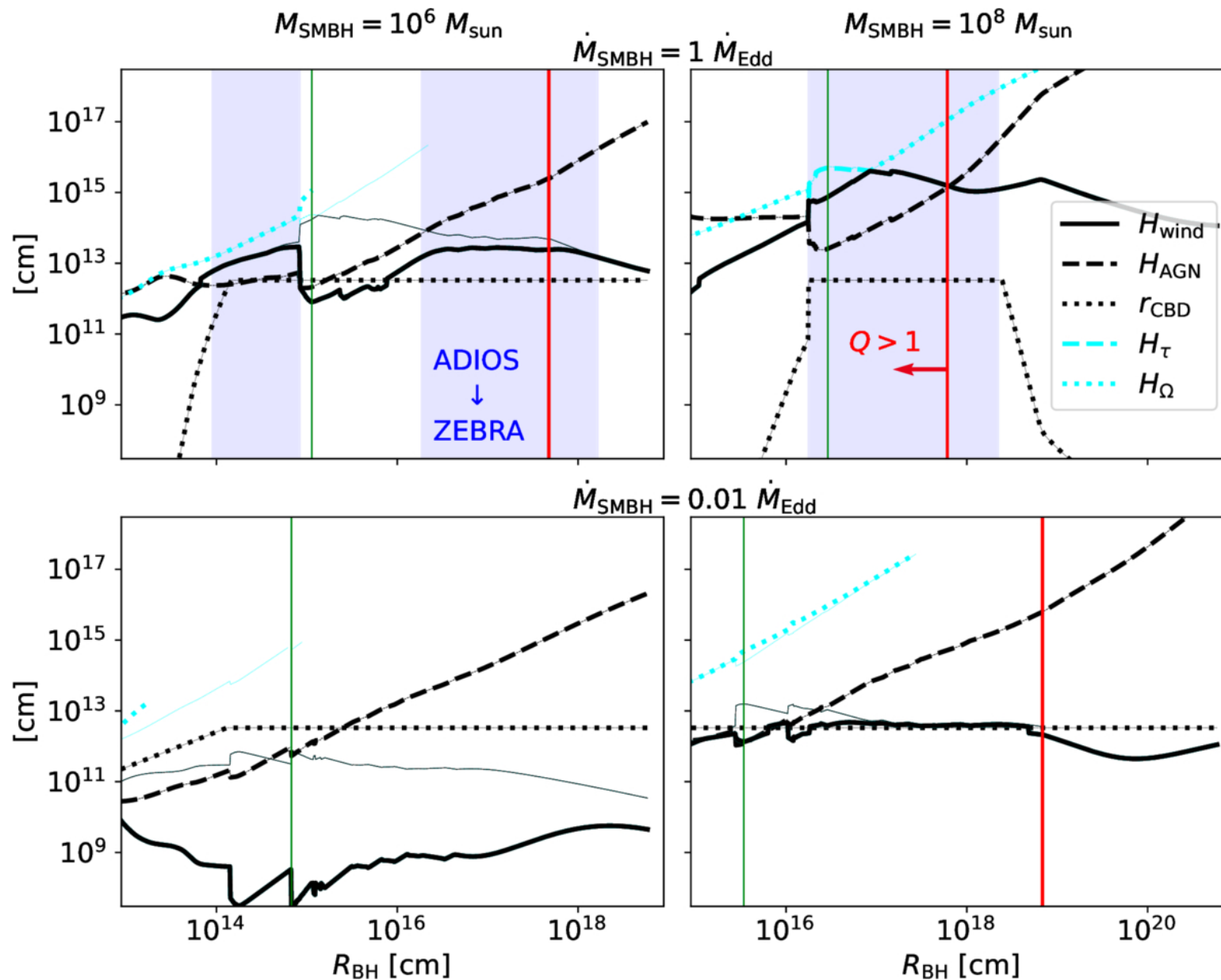
Figure 10. from Hiromichi Tagawa et al 2026 Astrophys. J. 1006 doi:10.3847/1538-4357/ae7d29 https://dx.doi.org/10.3847/1538-4357/ae7d29 © 2026. The Author(s). Published by the American Astronomical Society.
