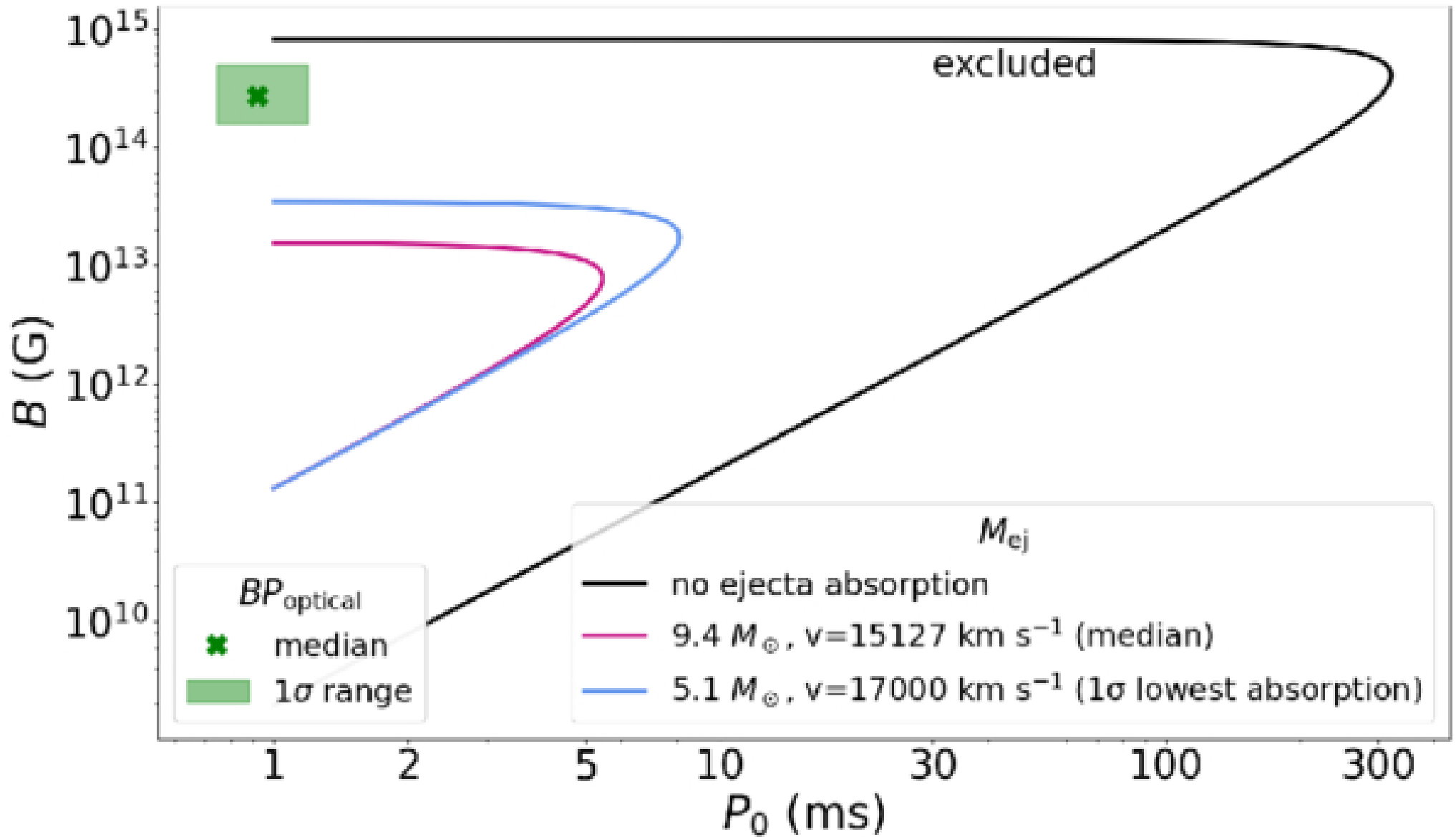
Figure 5. from Julia Ahlvind et al 2026 Astrophys. J. 1005 doi:10.3847/1538-4357/ae7c7a https://dx.doi.org/10.3847/1538-4357/ae7c7a © 2026. The Author(s). Published by the American Astronomical Society.
