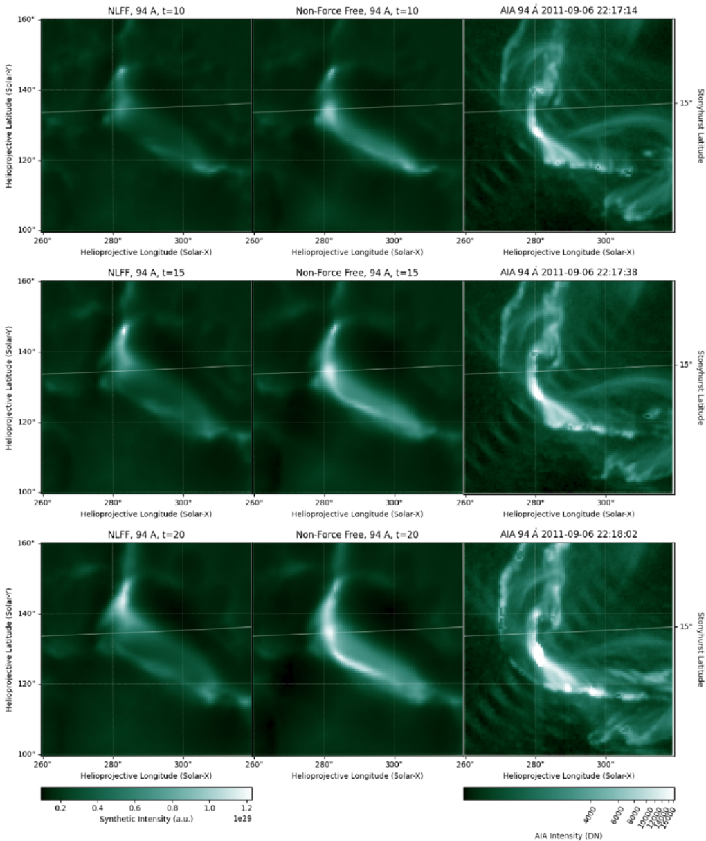
Figure 6. from W. Bate et al 2026 Astrophys. J. 1006 doi:10.3847/1538-4357/ae7c69 https://dx.doi.org/10.3847/1538-4357/ae7c69 © 2026. The Author(s). Published by the American Astronomical Society.
