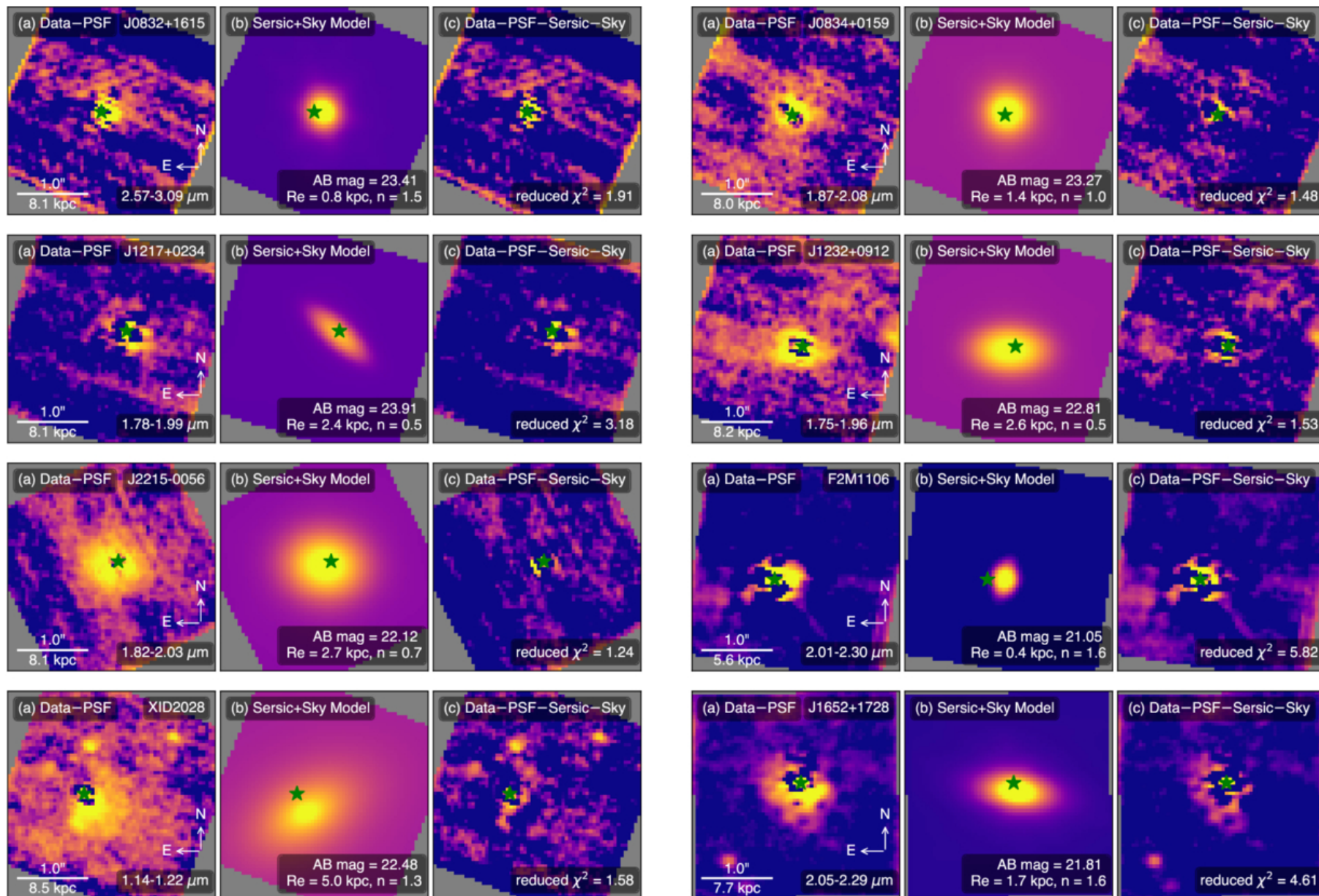
Figure 3. from Yu-Ching Chen et al 2026 Astrophys. J. 1006 doi:10.3847/1538-4357/ae7c01 https://dx.doi.org/10.3847/1538-4357/ae7c01 © 2026. The Author(s). Published by the American Astronomical Society.
