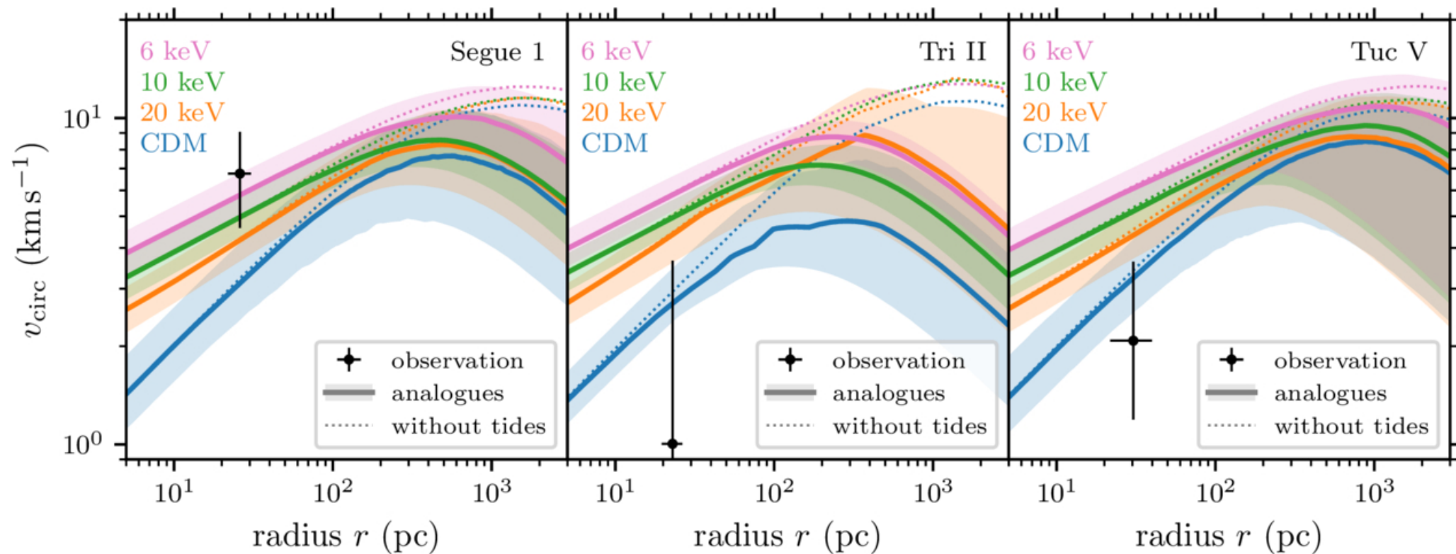
Figure 7. from M. Sten Delos et al 2026 Astrophys. J. 1006 doi:10.3847/1538-4357/ae7bed https://dx.doi.org/10.3847/1538-4357/ae7bed © 2026. The Author(s). Published by the American Astronomical Society.
