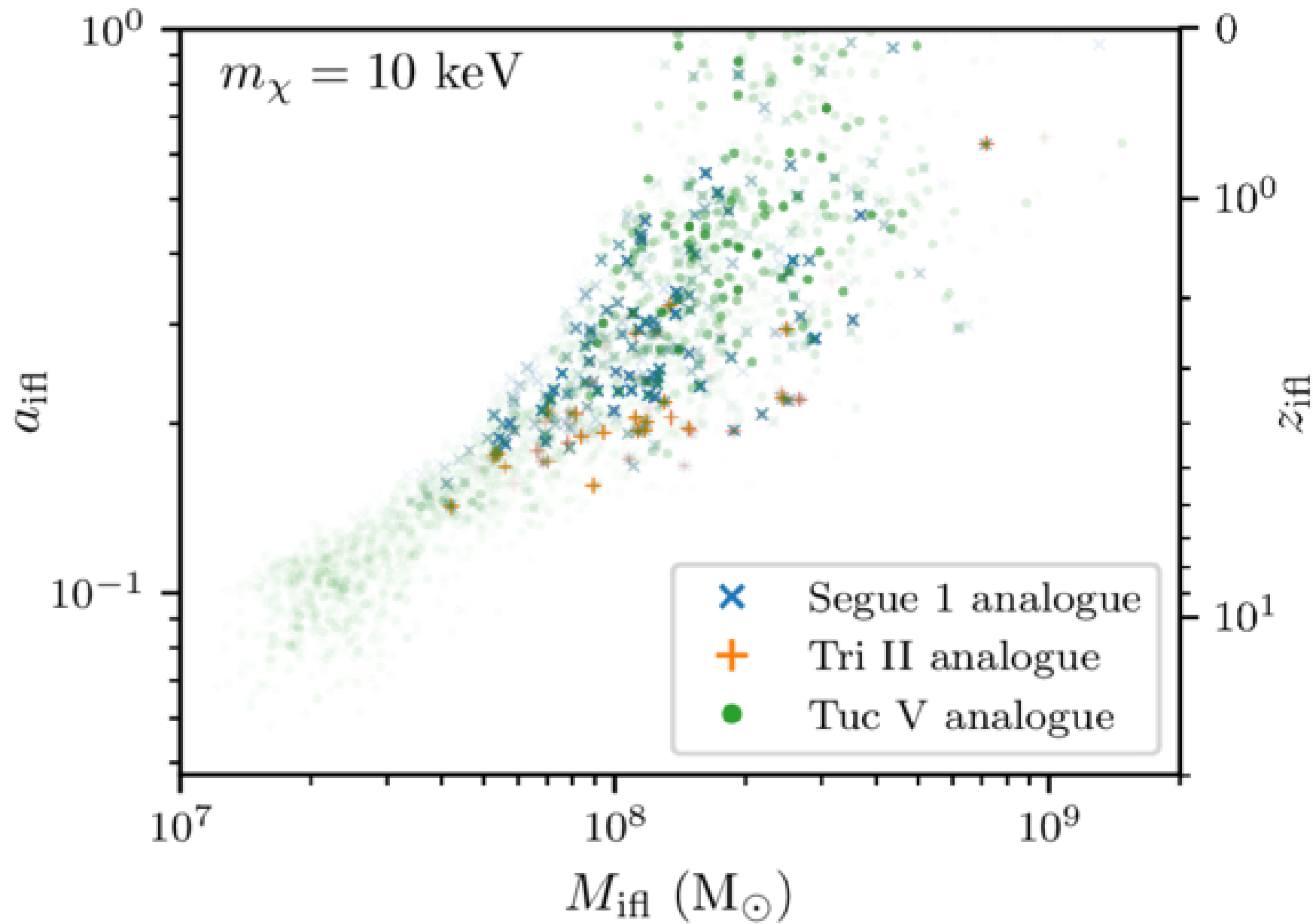
Figure 4. from M. Sten Delos et al 2026 Astrophys. J. 1006 doi:10.3847/1538-4357/ae7bed https://dx.doi.org/10.3847/1538-4357/ae7bed © 2026. The Author(s). Published by the American Astronomical Society.
