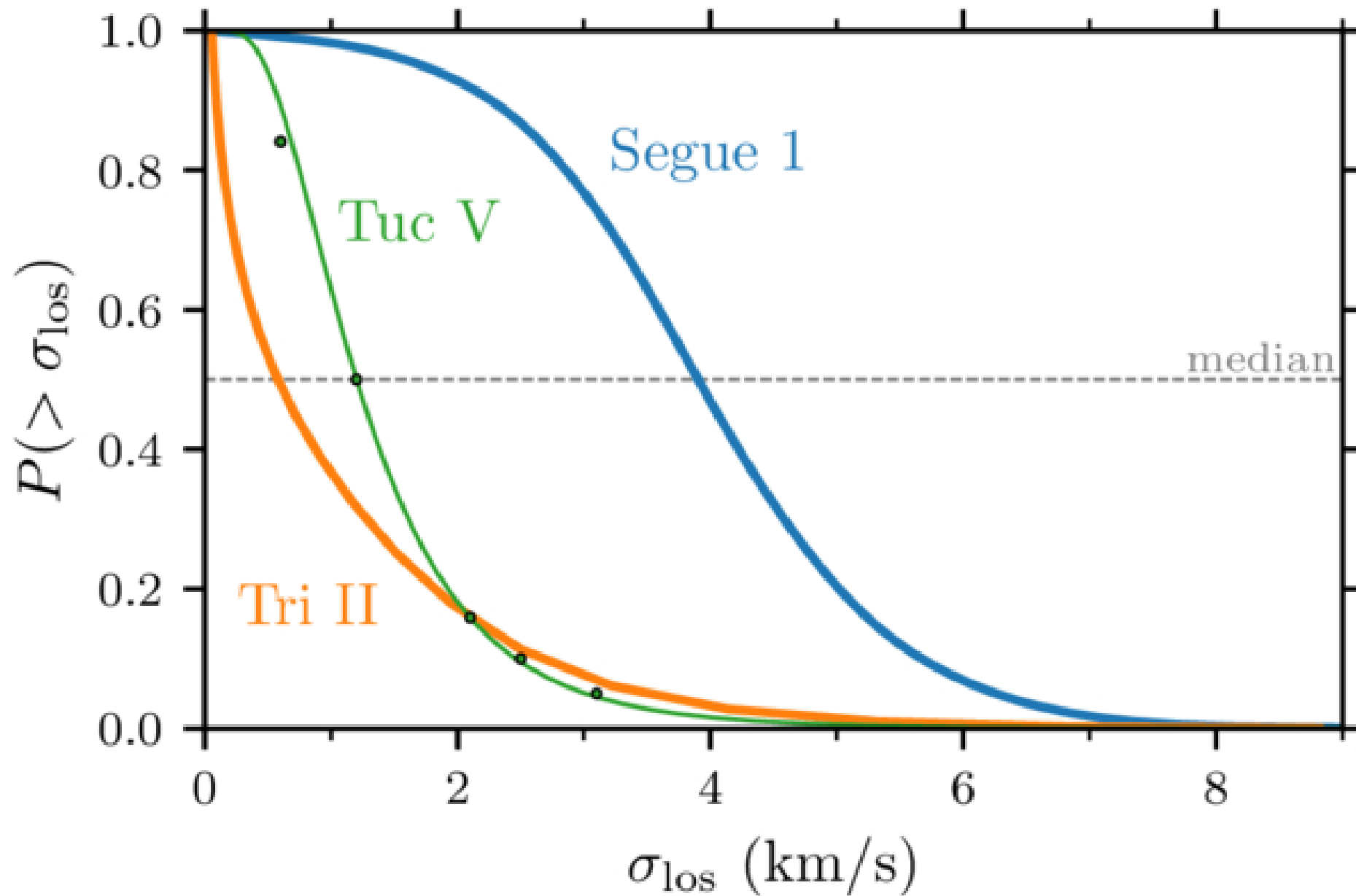
Figure 3. from M. Sten Delos et al 2026 Astrophys. J. 1006 doi:10.3847/1538-4357/ae7bed https://dx.doi.org/10.3847/1538-4357/ae7bed © 2026. The Author(s). Published by the American Astronomical Society.
