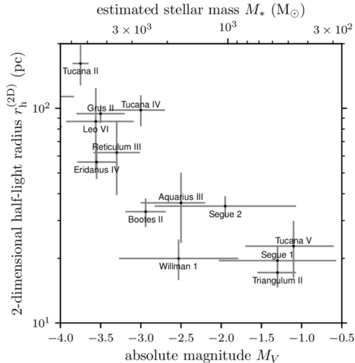
Figure 2. from M. Sten Delos et al 2026 Astrophys. J. 1006 doi:10.3847/1538-4357/ae7bed https://dx.doi.org/10.3847/1538-4357/ae7bed © 2026. The Author(s). Published by the American Astronomical Society.
