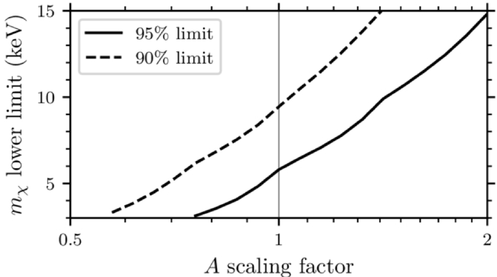
Figure 13. from M. Sten Delos et al 2026 Astrophys. J. 1006 doi:10.3847/1538-4357/ae7bed https://dx.doi.org/10.3847/1538-4357/ae7bed © 2026. The Author(s). Published by the American Astronomical Society.
