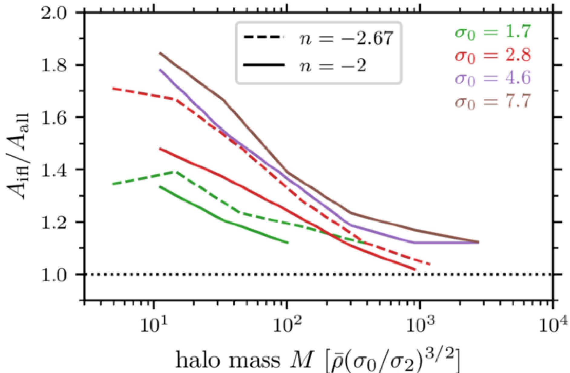
Figure 10. from M. Sten Delos et al 2026 Astrophys. J. 1006 doi:10.3847/1538-4357/ae7bed https://dx.doi.org/10.3847/1538-4357/ae7bed © 2026. The Author(s). Published by the American Astronomical Society.
